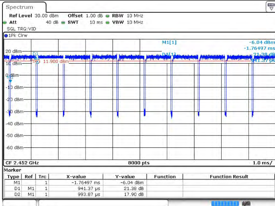
11N40SISO Ant9 2452
