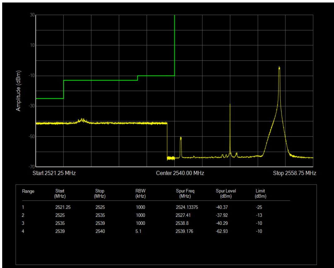
Band41 QAM16 BW=15MHz Channel=40165 RB Size=75 Position=#0
