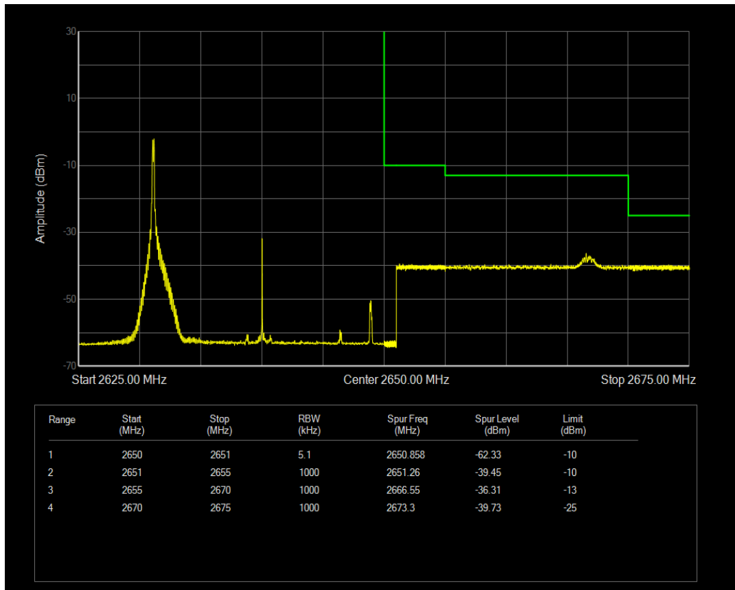
Band41 QAM16 BW=20MHz Channel=41090 RB Size=1 Position=#Max
