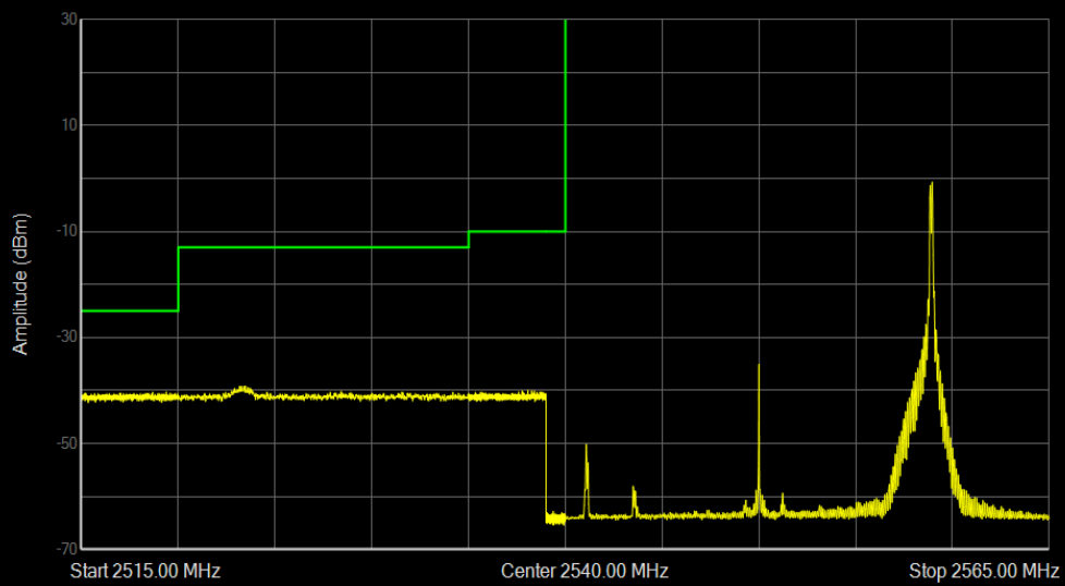
Band41 QPSK BW=20MHz Channel=40190 RB Size=1 Position=#Max
