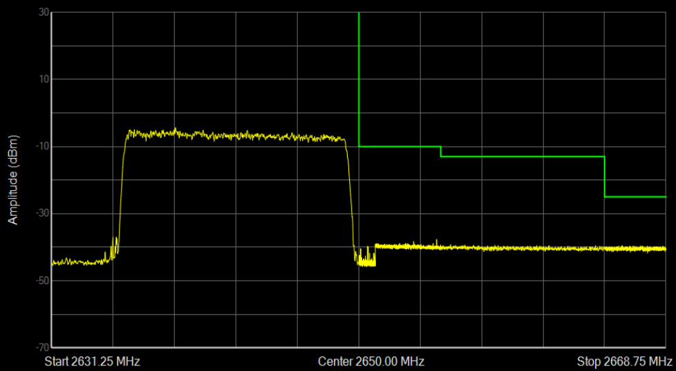
Band41 QAM16 BW=15MHz Channel=41115 RB Size=75 Position=#0
