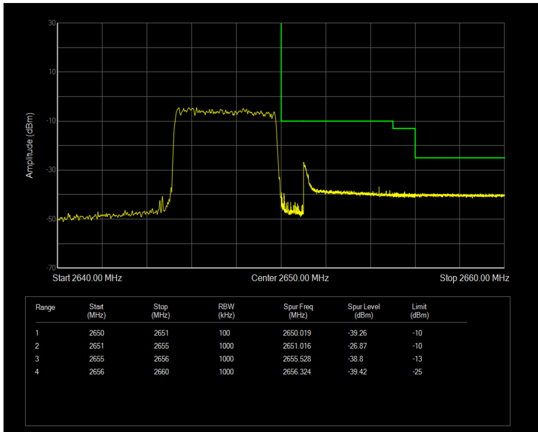
Band41 QAM16 BW=5MHz Channel=41165 RB Size=1 Position=#Max
