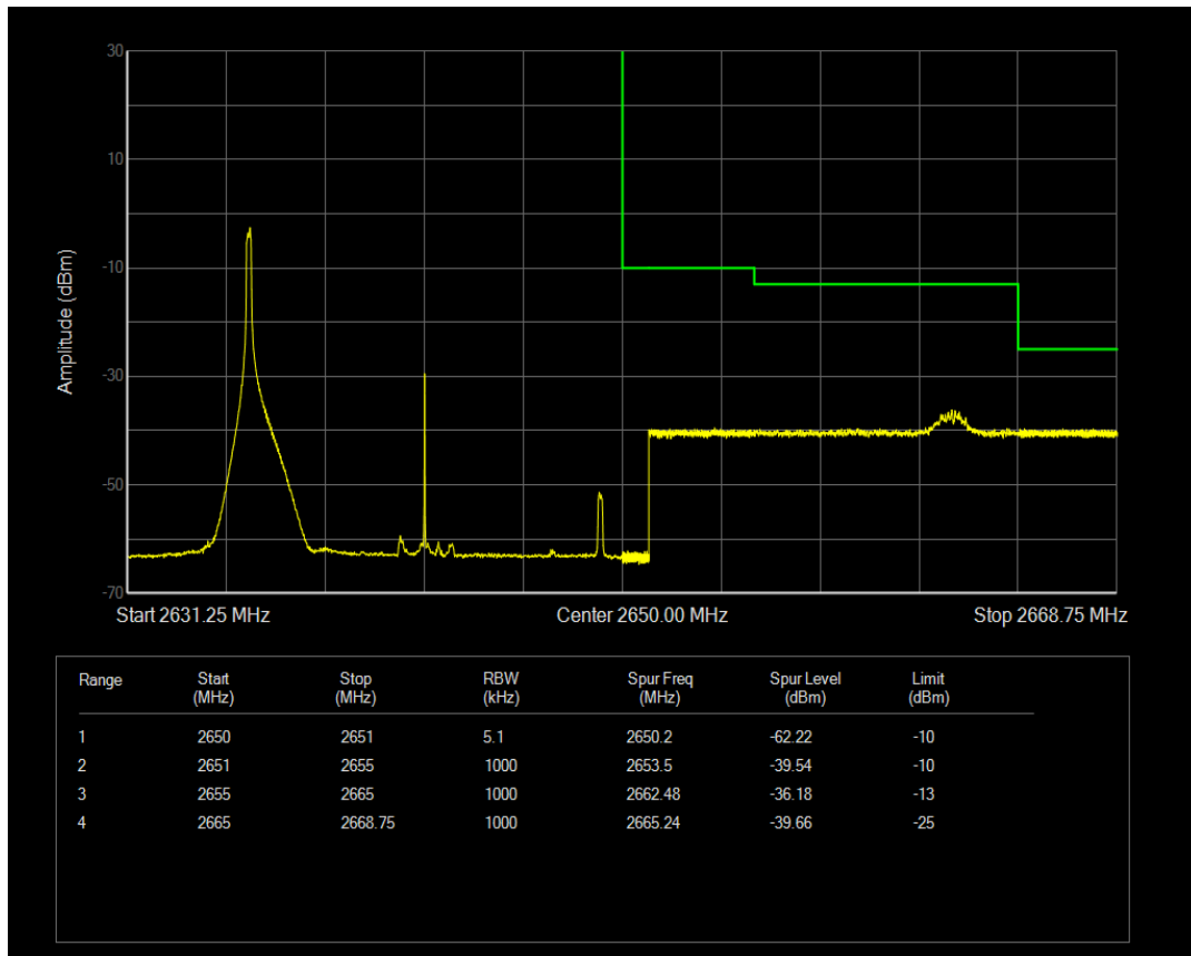
Band41 QAM16 BW=15MHz Channel=41115 RB Size=1 Position=#0
