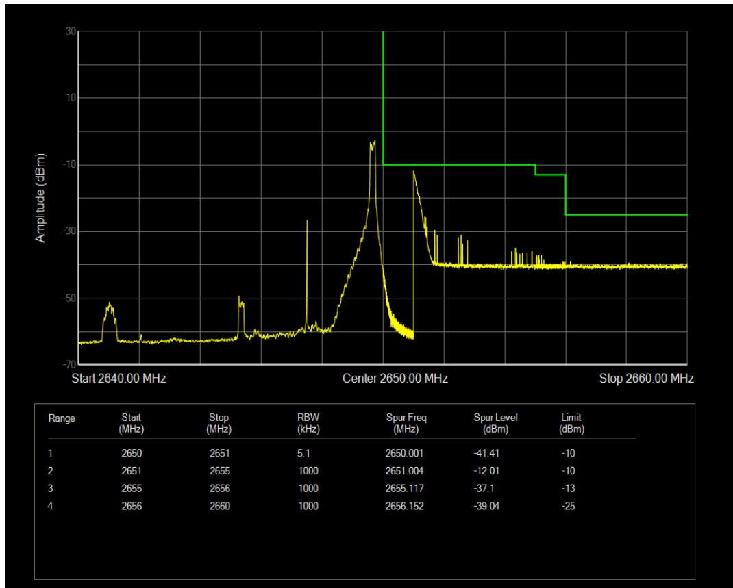
Band41 QAM16 BW=5MHz Channel=41165 RB Size=1 Position=#0
