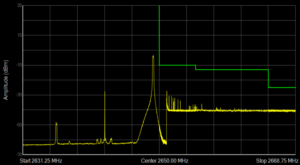
Band41 QPSK BW=15MHz Channel=41115 RB Size=1 Position=#Max
