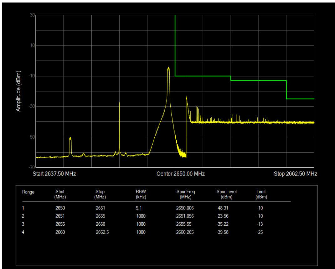
Band41 QAM16 BW=10MHz Channel=41140 RB Size=50 Position=#0
