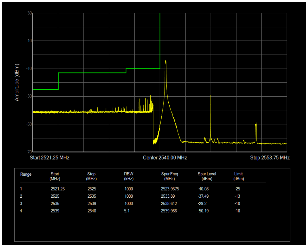
Band41 QAM16 BW=15MHz Channel=40165 RB Size=1 Position=#Max
