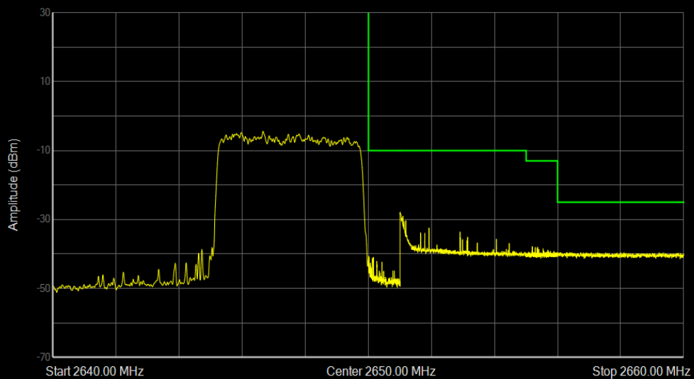
Band41 QAM16 BW=5MHz Channel=41165 RB Size=25 Position=#0
