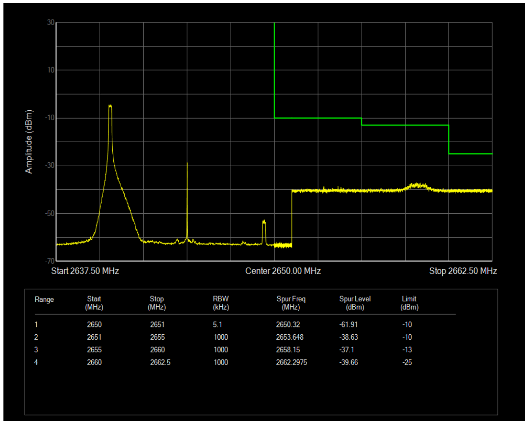
Band41 QAM16 BW=10MHz Channel=41140 RB Size=1 Position=#Max
