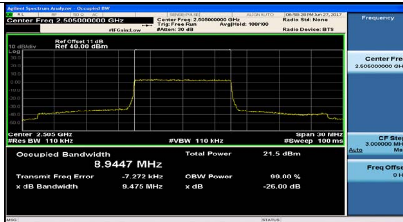
Band7_10MHz_16QAM_20800_50RB#0
