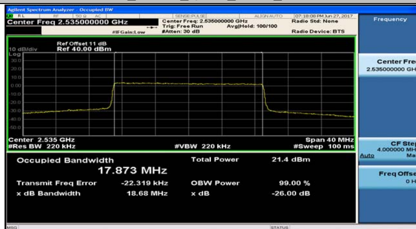
Band7_20MHz_16QAM_21100_100RB#0
