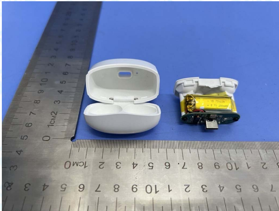
Photo 12 Appearance of PCB &amp; Battery
