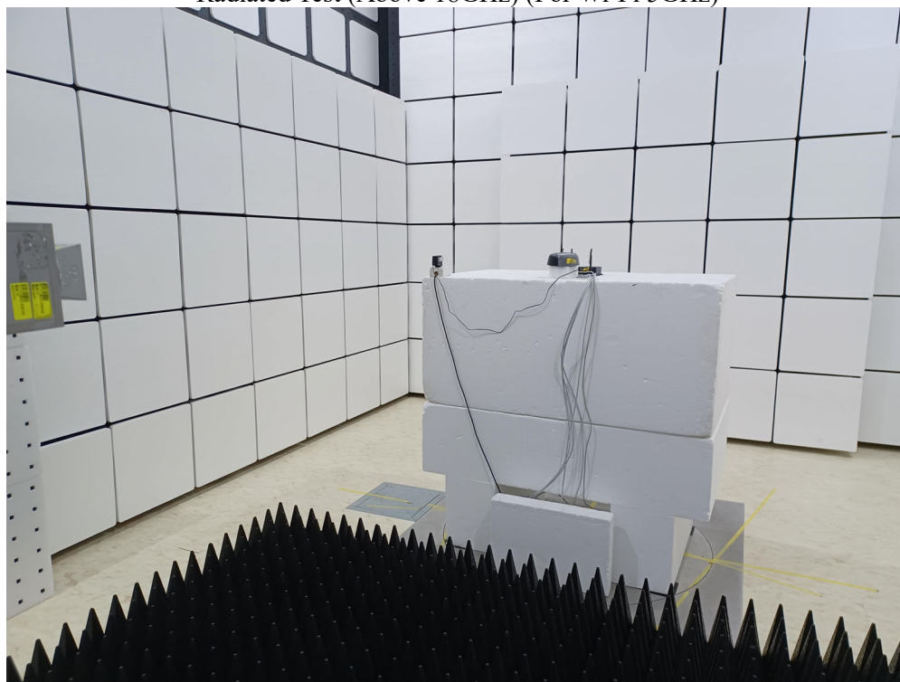
Radiated Test (Above 18GHz) (For Wi-Fi 5GHz)
