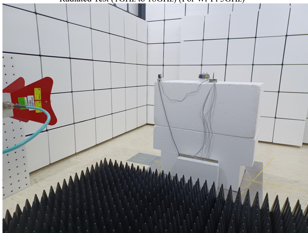
Radiated Test (1GHz to 18GHz) (For Wi-Fi 5GHz)
