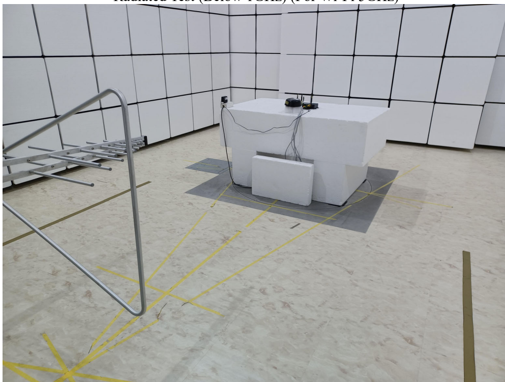
Radiated Test (Below 1GHz) (For Wi-Fi 5GHz)
