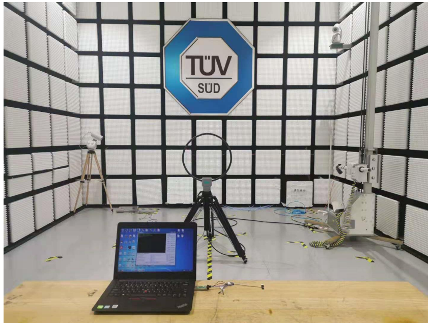
Radiated Emission Setup 9kHz ~ 30MHz
