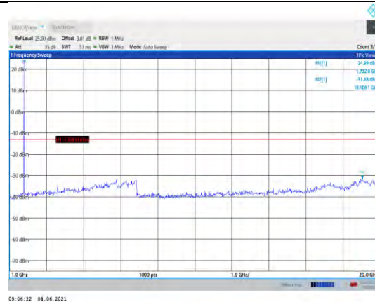
Band4-3MHz-16QAM-20175-1RB#0- Range2:1000~20000MHz
