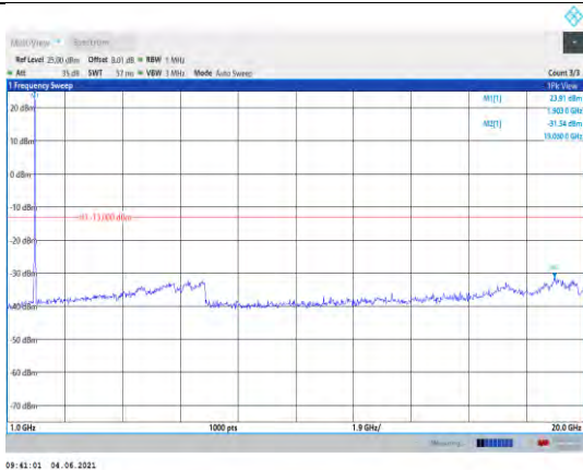
Band25-15MHz-16QAM-26615-1RB#0- Range2:1000~20000MHz
