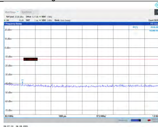
Band4-3MHz-16QAM-20385-1RB#0- Range1:30~1000MHz
