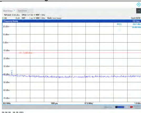
Band25-1.4MHz-16QAM-26047-1RB#0- Range1:30~1000MHz
