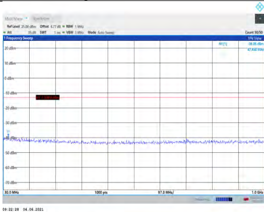
Band4-20MHz-16QAM-20175-1RB#0- Range1:30~1000MHz
