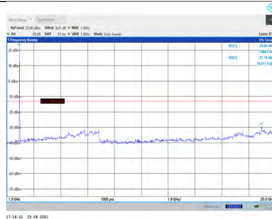
Band2-10MHz-QPSK-18900-1RB#0- Range2:1000~20000MHz
