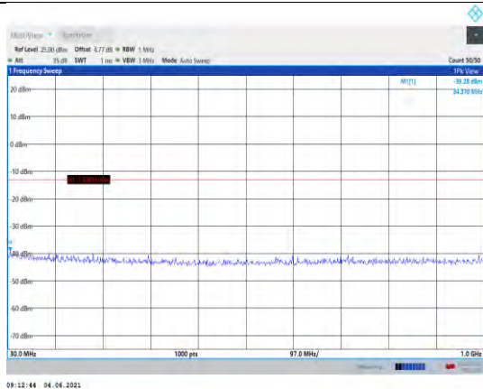
Band4-10MHz-16QAM-20000-1RB#0- Range1:30~1000MHz
