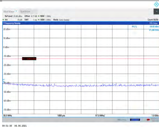
Band4-1.4MHz-QPSK-19957-1RB#0- Range1:30~1000MHz
