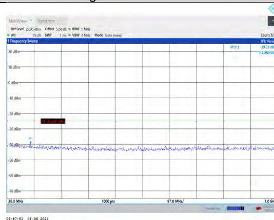
Band41-5MHz-QPSK-40620-1RB#0- Range1:30~1000MHz
