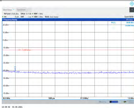
Band2-1.4MHz-16QAM-18607-1RB#0- Range1:30~1000MHz
