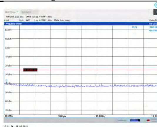
Band41-10MHz-QPSK-40620-1RB#0-Range1:30~1000MHz
