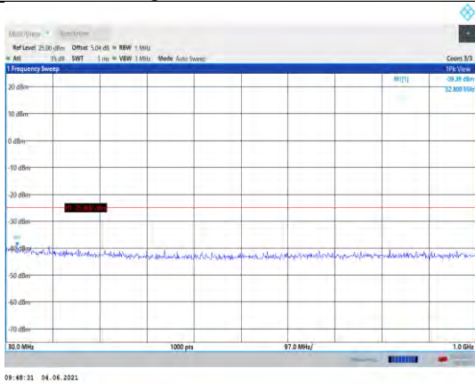
Band41-5MHz-16QAM-40620-1RB#0- Range1:30~1000MHz
