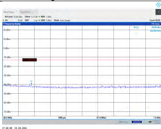
Band2-20MHz-QPSK-18900-1RB#0- Range1:30~1000MHz
