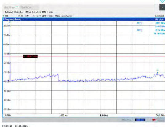
Band25-15MHz-16QAM-26115-1RB#0- Range2:1000~20000MHz
