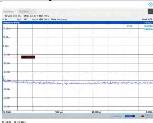
Band4-10MHz-16QAM-20175-1RB#0- Range1:30~1000MHz
