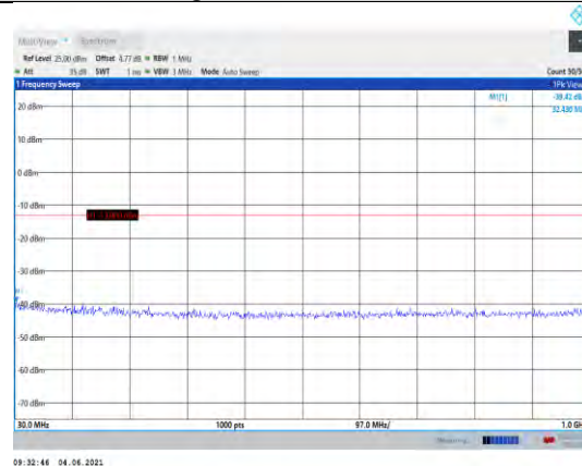
Band25-5MHz-QPSK-26665-1RB#0- Range1:30~1000MHz
