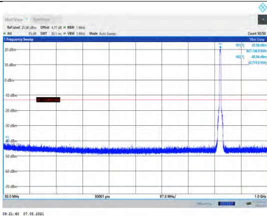
Band5-4132-30~1000MHz
