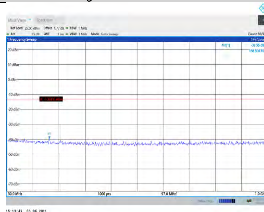
Band2-1.4MHz-16QAM-19193-1RB#0- Range1:30~1000MHz
