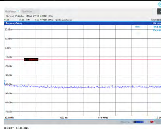
Band25-1.4MHz-16QAM-26683-1RB#0- Range1:30~1000MHz
