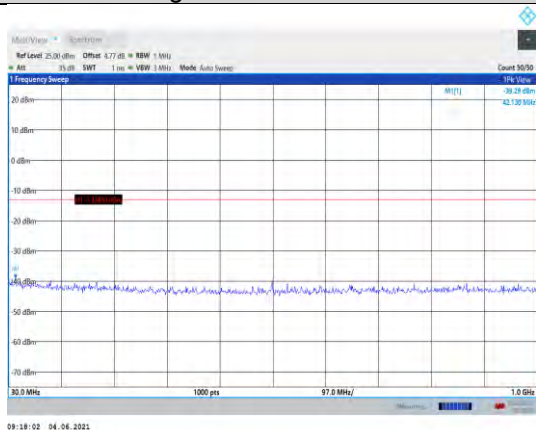
Band4-15MHz-16QAM-20175-1RB#0- Range1:30~1000MHz
