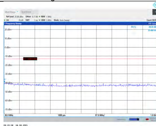
Band4-10MHz-16QAM-20350-1RB#0- Range1:30~1000MHz
