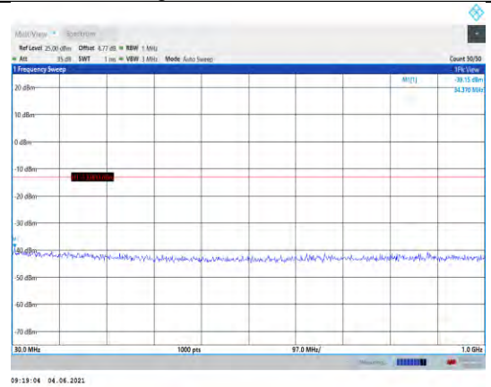
Band4-15MHz-QPSK-20325-1RB#0- Range1:30~1000MHz
