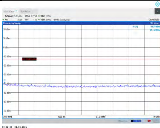
Band4-1.4MHz-QPSK-20175-1RB#0- Range1:30~1000MHz
