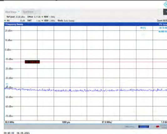
Band25-20MHz-16QAM-26590-1RB#0- Range1:30~1000MHz
