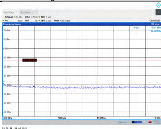
Band25-15MHz-QPSK-26115-1RB#0- Range1:30~1000MHz
