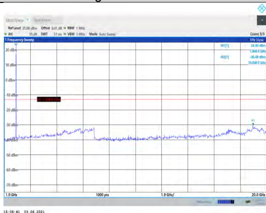
Band2-1.4MHz-16QAM-18607-1RB#0- Range2:1000~20000MHz
