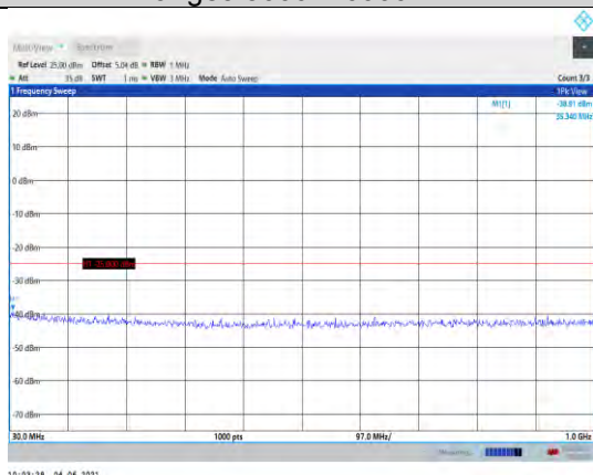
Band41-10MHz-QPSK-41540-1RB#0- Range1:30~1000MHz
