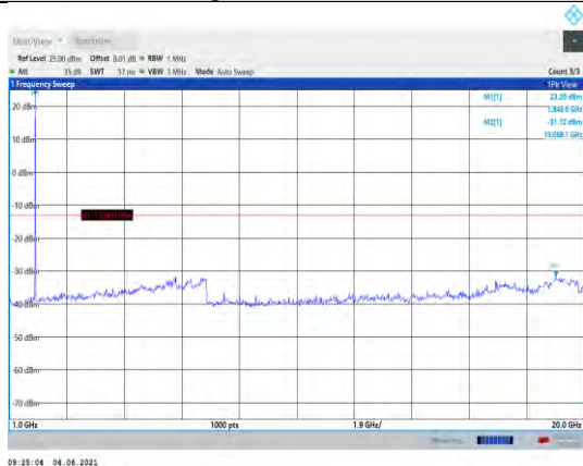
Band25-1.4MHz-16QAM-26047-1RB#0- Range2:1000~20000MHz
