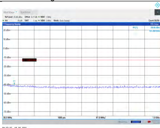
Band25-3MHz-QPSK-26055-1RB#0- Range1:30~1000MHz
