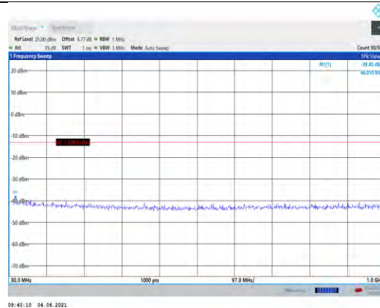
Band25-15MHz-16QAM-26365-1RB#0- Range1:30~1000MHz
