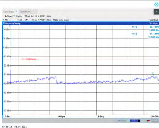
Band25-5MHz-16QAM-26665-1RB#0- Range2:1000~20000MHz
