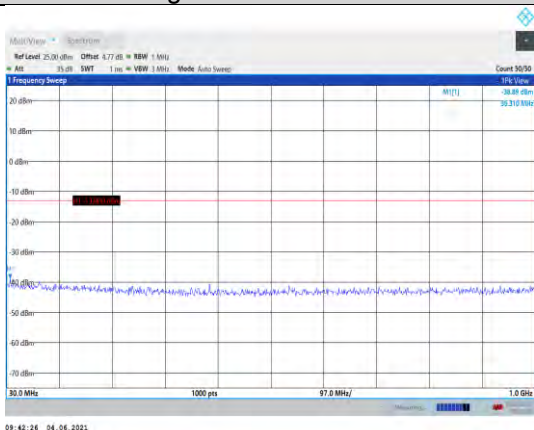
Band25-20MHz-QPSK-26140-1RB#0- Range1:30~1000MHz
