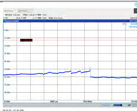
Band5-4182-3000~10000MHz
