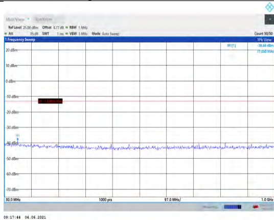
Band4-15MHz-QPSK-20175-1RB#0- Range1:30~1000MHz
