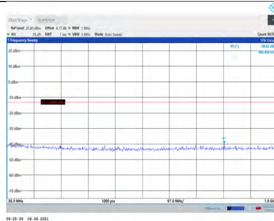
Band25-1.4MHz-16QAM-26365-1RB#0- Range1:30~1000MHz
