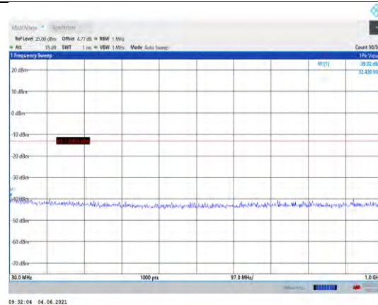
Band25-5MHz-QPSK-26365-1RB#0- Range1:30~1000MHz
