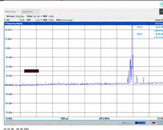
Band41-10MHz-QPSK-40620-1RB#0-Range2:1000~3000MHz
