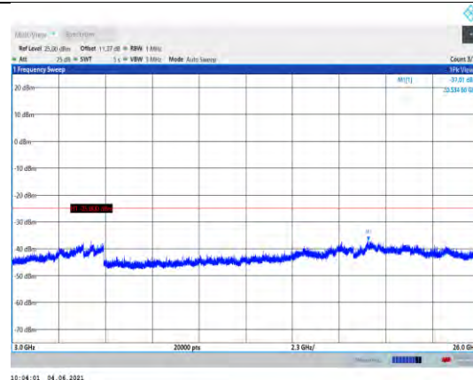
Band41-10MHz-QPSK-41540-1RB#0- Range3:3000~26000MHz
