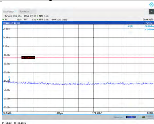
Band2-10MHz-QPSK-18900-1RB#0- Range1:30~1000MHz
