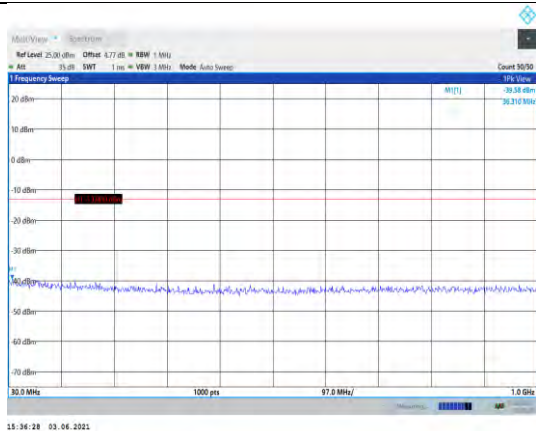
Band2-5MHz-QPSK-18625-1RB#0- Range1:30~1000MHz
