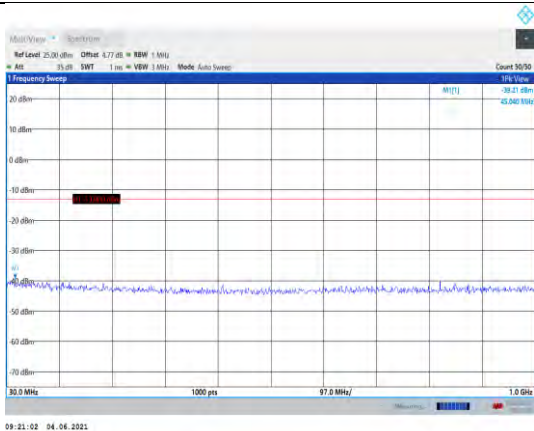
Band4-20MHz-QPSK-20050-1RB#0- Range1:30~1000MHz
