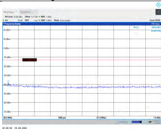
Band2-3MHz-QPSK-18900-1RB#0-Range1:30~1000MHz
