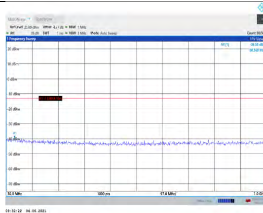
Band25-5MHz-16QAM-26365-1RB#0- Range1:30~1000MHz
