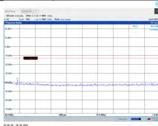
Band25-15MHz-QPSK-26615-1RB#0- Range1:30~1000MHz
