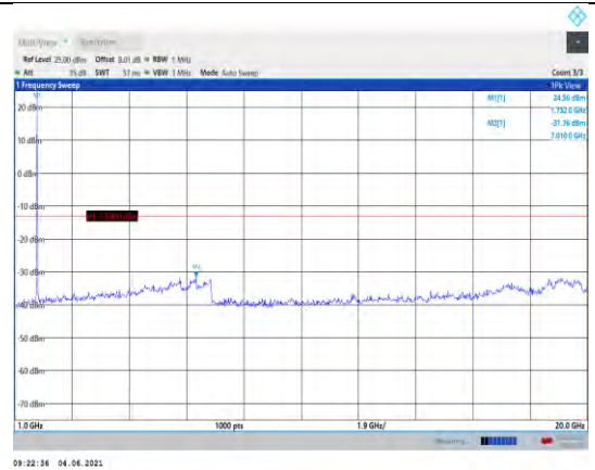
Band4-20MHz-16QAM-20175-1RB#0- Range2:1000~20000MHz
