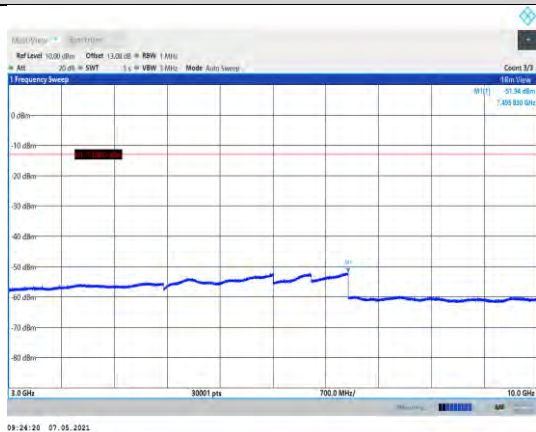
Band5-4233-3000~10000MHz
