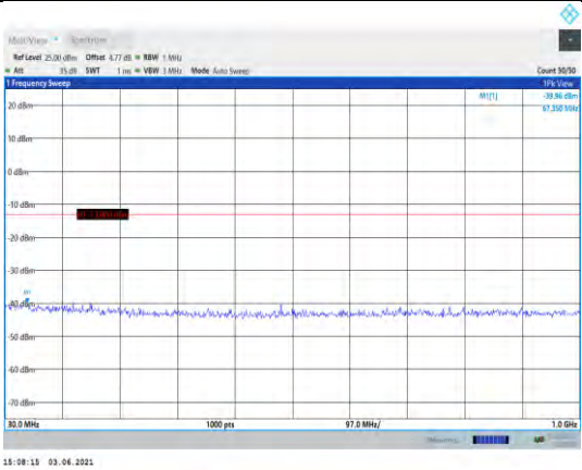
Band2-1.4MHz-QPSK-18607-1RB#0- Range1:30~1000MHz
