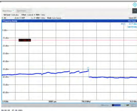
Band5-4132-3000~10000MHz
