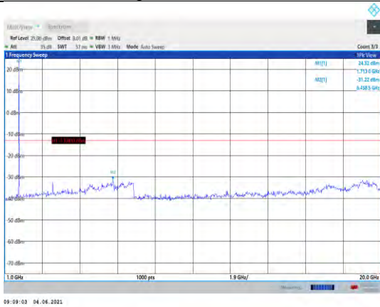
Band4-5MHz-16QAM-19975-1RB#0- Range2:1000~20000MHz
