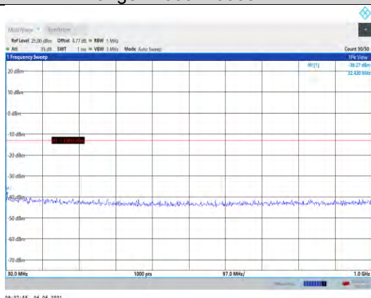
Band25-3MHz-16QAM-26055-1RB#0- Range1:30~1000MHz
