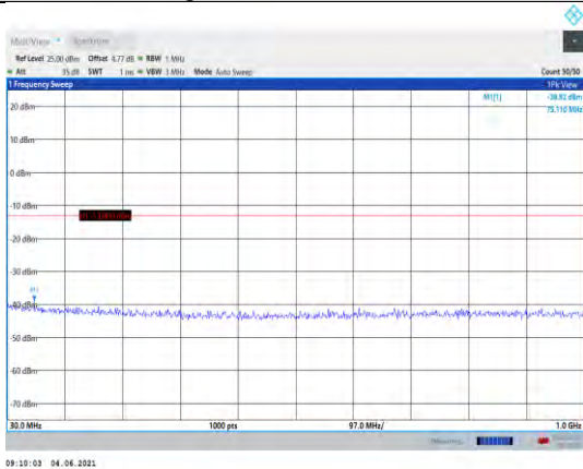
Band4-5MHz-16QAM-20175-1RB#0- Range1:30~1000MHz
