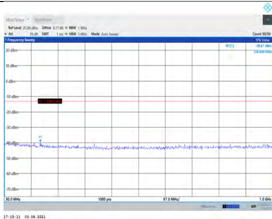
Band2-10MHz-QPSK-18650-1RB#0- Range1:30~1000MHz
