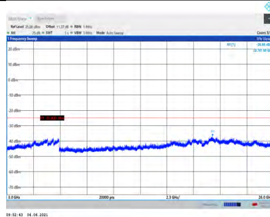
Band41-10MHz-QPSK-39700-1RB#0-Range3:3000~26000MHz
