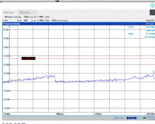
Band2-10MHz-16QAM-18650-1RB#0- Range2:1000~20000MHz
