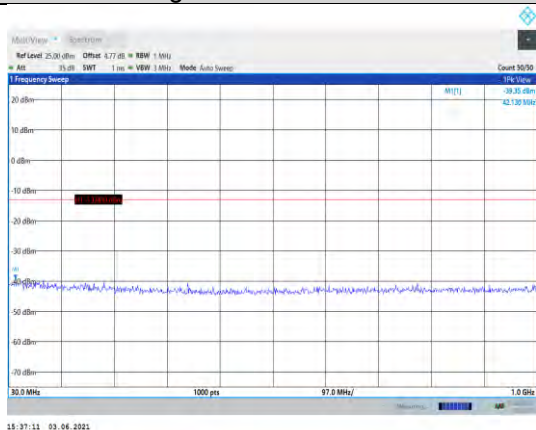
Band2-5MHz-QPSK-18900-1RB#0- Range1:30~1000MHz
