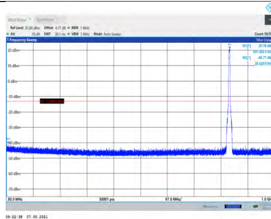
Band5-4182-30~1000MHz
