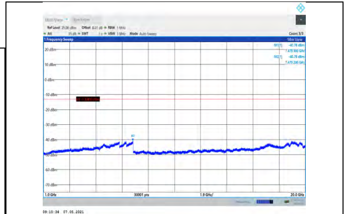
Band2-9400-1000~20000MHz
