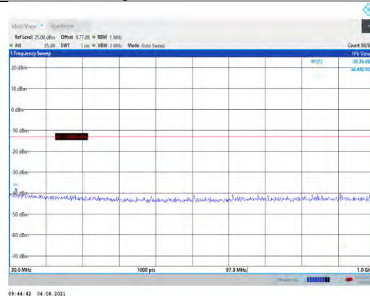
Band25-20MHz-QPSK-26590-1RB#0- Range1:30~1000MHz
