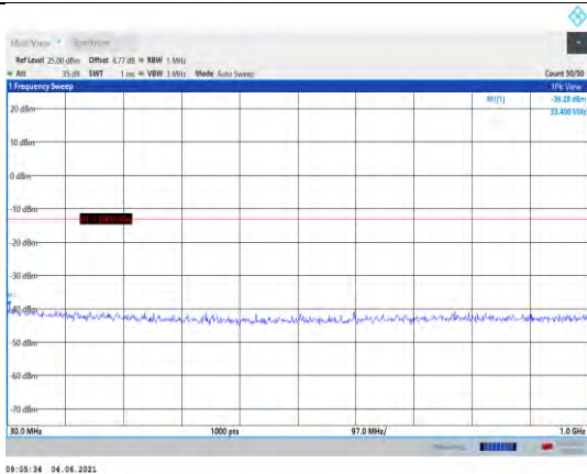
Band4-3MHz-16QAM-19965-1RB#0- Range1:30~1000MHz
