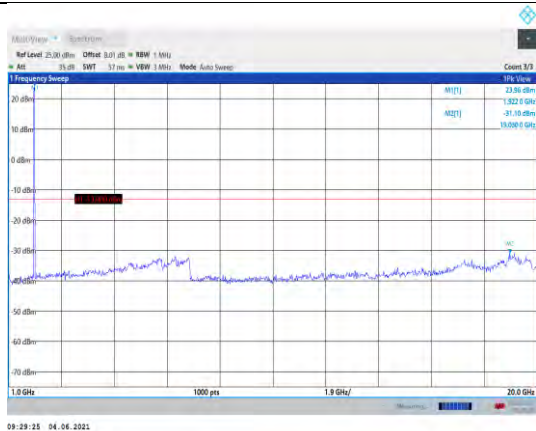
Band25-3MHz-16QAM-26675-1RB#0- Range2:1000~20000MHz
