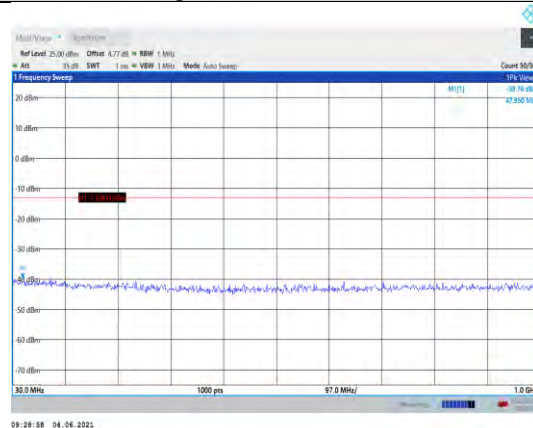
Band25-3MHz-QPSK-26675-1RB#0- Range1:30~1000MHz
