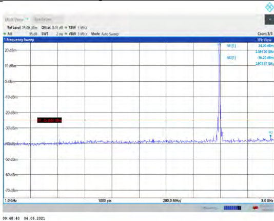
Band41-5MHz-16QAM-40620-1RB#0- Range2:1000~3000MHz
