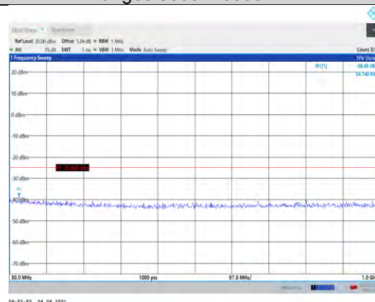
Band41-10MHz-16QAM-39700-1RB#0- Range1:30~1000MHz
