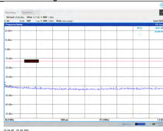
Band2-3MHz-QPSK-19185-1RB#0-Range1:30~1000MHz
