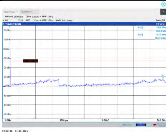
Band25-20MHz-16QAM-26140-1RB#0- Range2:1000~20000MHz
