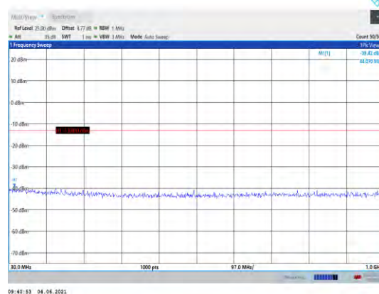
Band25-15MHz-16QAM-26615-1RB#0- Range1:30~1000MHz
