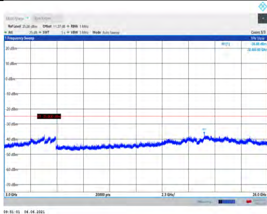
Band41-5MHz-16QAM-41565-1RB#0-Range3:3000~26000MHz
