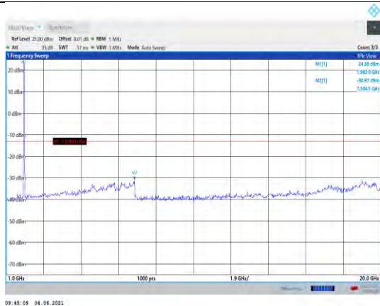
Band25-20MHz-16QAM-26590-1RB#0- Range2:1000~20000MHz
