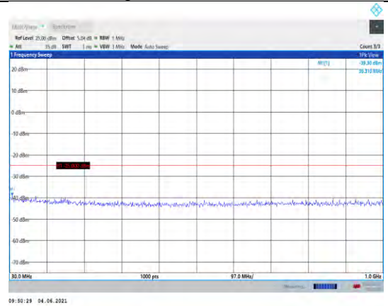
Band41-5MHz-16QAM-41565-1RB#0- Range1:30~1000MHz
