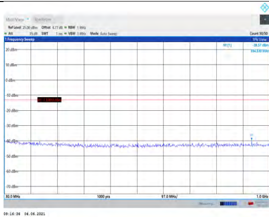
Band4-15MHz-QPSK-20025-1RB#0- Range1:30~1000MHz
