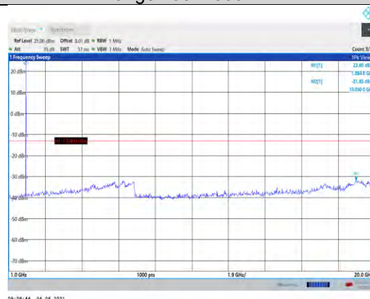
Band25-3MHz-16QAM-26365-1RB#0- Range2:1000~20000MHz
