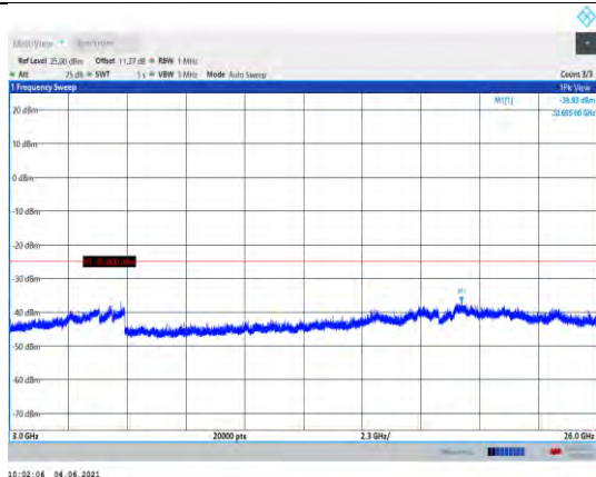
Band41-10MHz-QPSK-40620-1RB#0- Range3:3000~26000MHz
