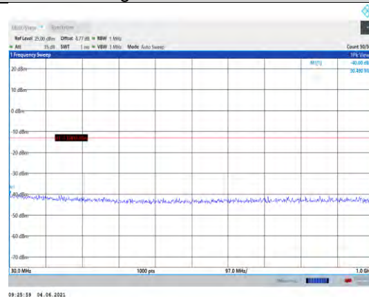
Band25-1.4MHz-QPSK-26683-1RB#0- Range1:30~1000MHz
