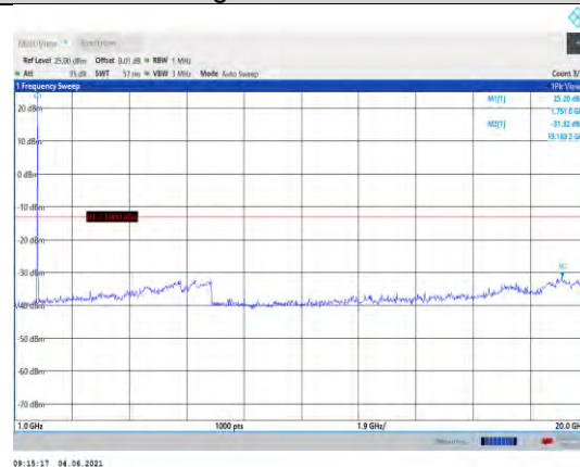
Band4-10MHz-16QAM-20350-1RB#0- Range2:1000~20000MHz
