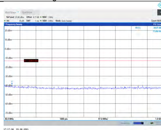
Band2-10MHz-QPSK-19150-1RB#0- Range1:30~1000MHz
