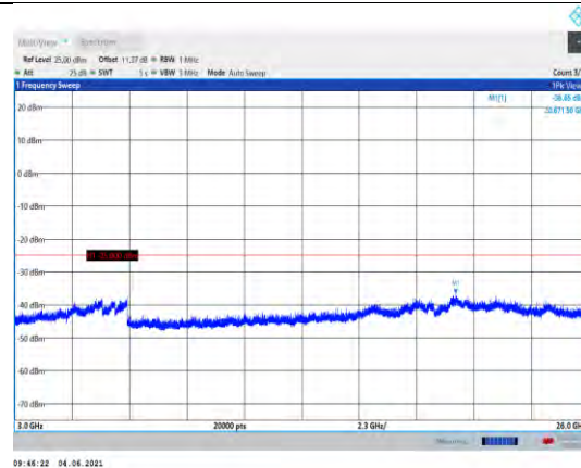
Band41-5MHz-QPSK-39675-1RB#0- Range3:3000~26000MHz
