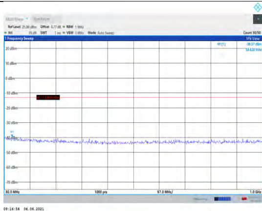
Band4-15MHz-16QAM-20025-1RB#0- Range1:30~1000MHz
