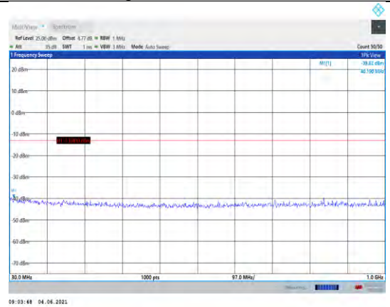
Band4-1.4MHz-16QAM-20393-1RB#0- Range1:30~1000MHz
