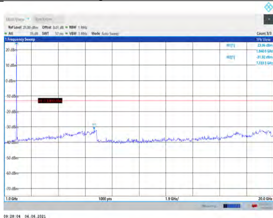
Band25-3MHz-16QAM-26055-1RB#0- Range2:1000~20000MHz
