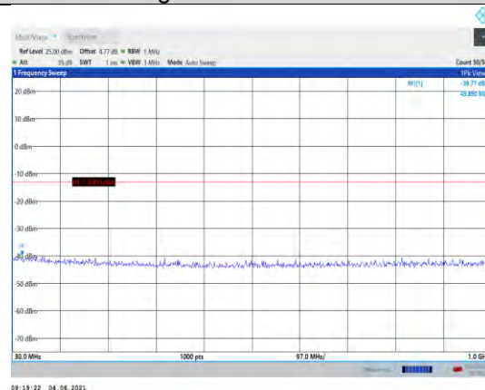
Band4-15MHz-16QAM-20325-1RB#0- Range1:30~1000MHz
