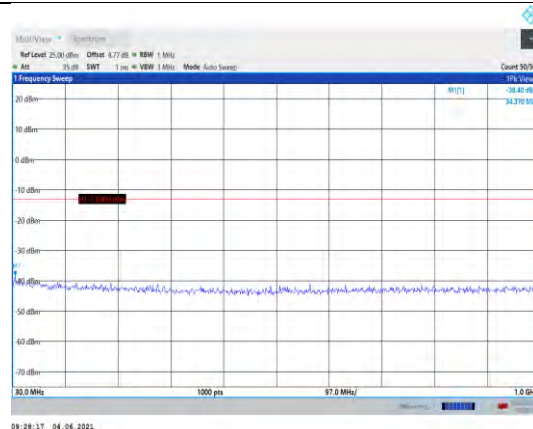
Band25-3MHz-QPSK-26365-1RB#0- Range1:30~1000MHz
