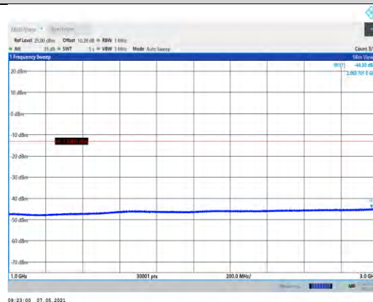
Band5-4182-1000~3000MHz
