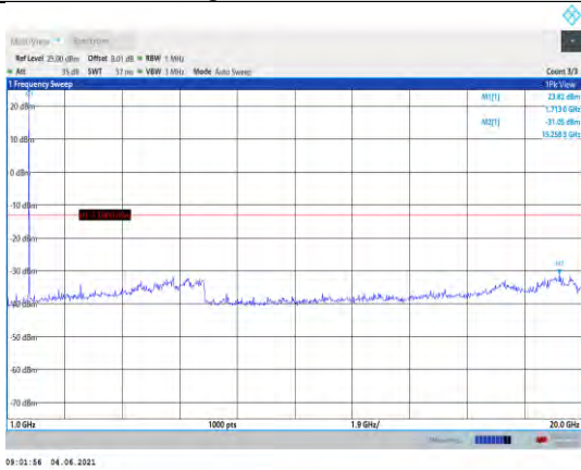
Band4-1.4MHz-16QAM-19957-1RB#0- Range2:1000~20000MHz
