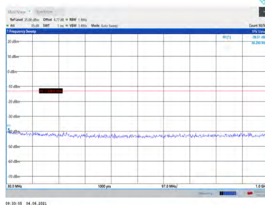
Band25-5MHz-16QAM-26665-1RB#0- Range1:30~1000MHz
