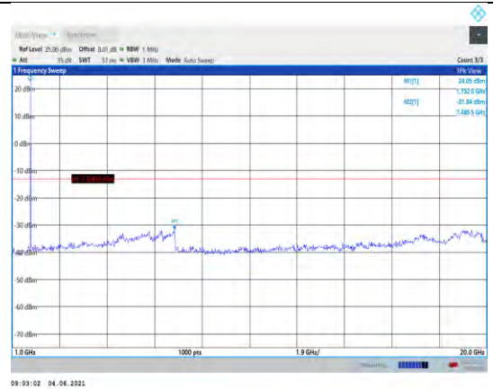
Band4-1.4MHz-16QAM-20175-1RB#0- Range2:1000~20000MHz
