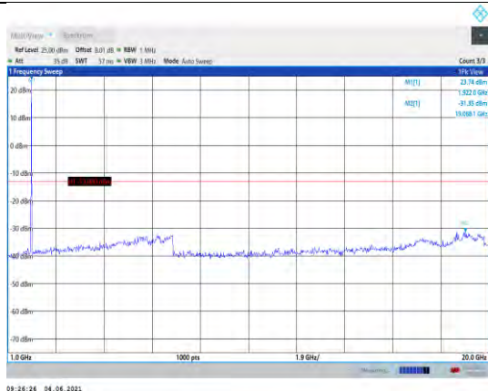
Band25-1.4MHz-16QAM-26683-1RB#0- Range2:1000~20000MHz
