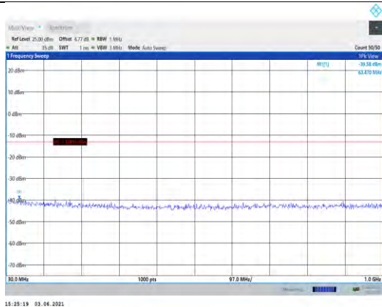
Band2-3MHz-QPSK-18615-1RB#0-Range1:30~1000MHz
