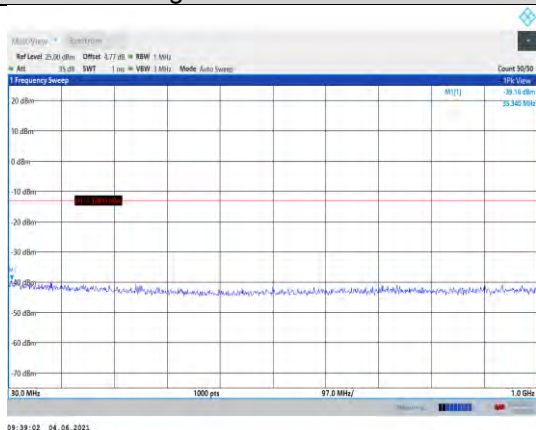
Band25-15MHz-16QAM-26115-1RB#0- Range1:30~1000MHz
