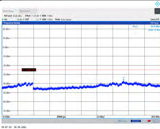
Band41-5MHz-16QAM-39675-1RB#0- Range3:3000~26000MHz
