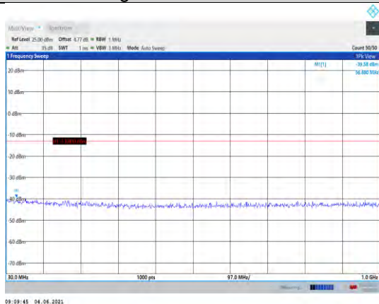
Band4-5MHz-QPSK-20175-1RB#0- Range1:30~1000MHz
