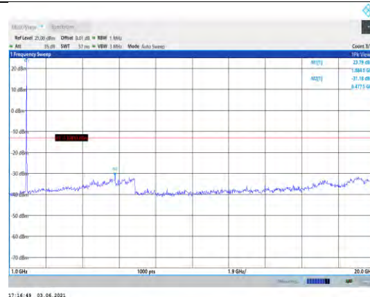
Band2-10MHz-16QAM-18900-1RB#0- Range2:1000~20000MHz
