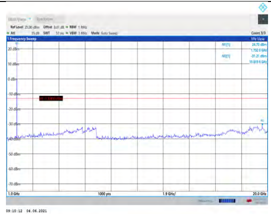
Band4-5MHz-16QAM-20175-1RB#0- Range2:1000~20000MHz
