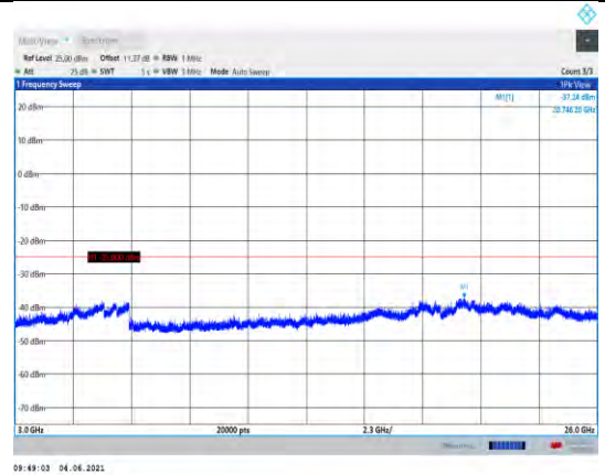
Band41-5MHz-16QAM-40620-1RB#0- Range3:3000~26000MHz
