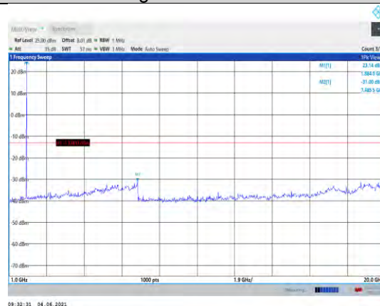
Band25-5MHz-16QAM-26365-1RB#0- Range2:1000~20000MHz
