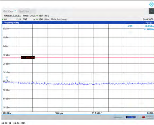
Band4-5MHz-16QAM-19975-1RB#0- Range1:30~1000MHz
