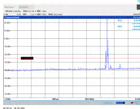
Band41-10MHz-16QAM-39700-1RB#0- Range2:1000~3000MHz
