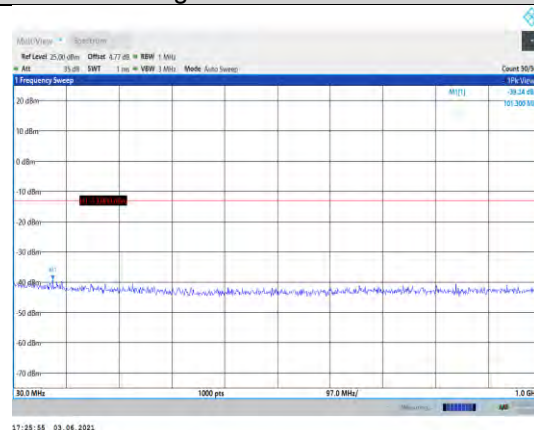
Band2-20MHz-QPSK-19100-1RB#0- Range1:30~1000MHz
