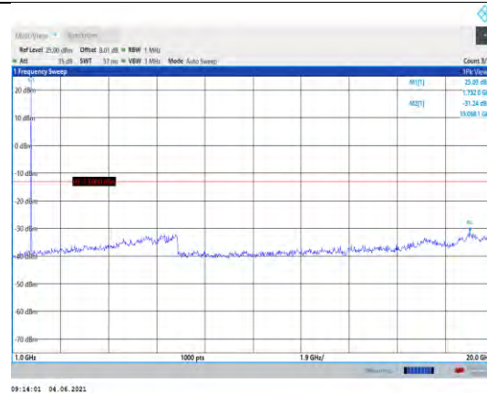
Band4-10MHz-16QAM-20175-1RB#0- Range2:1000~20000MHz
