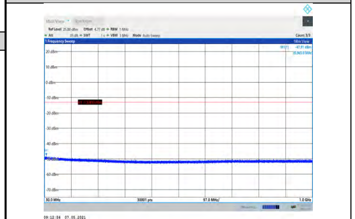
Band2-9538-30~1000MHz
