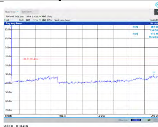
Band2-10MHz-16QAM-19150-1RB#0- Range2:1000~20000MHz
