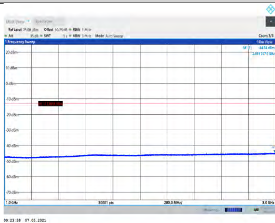
Band5-4233-1000~3000MHz
