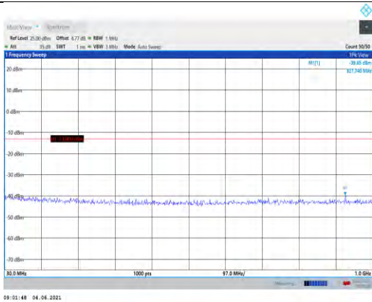
Band4-1.4MHz-16QAM-19957-1RB#0- Range1:30~1000MHz
