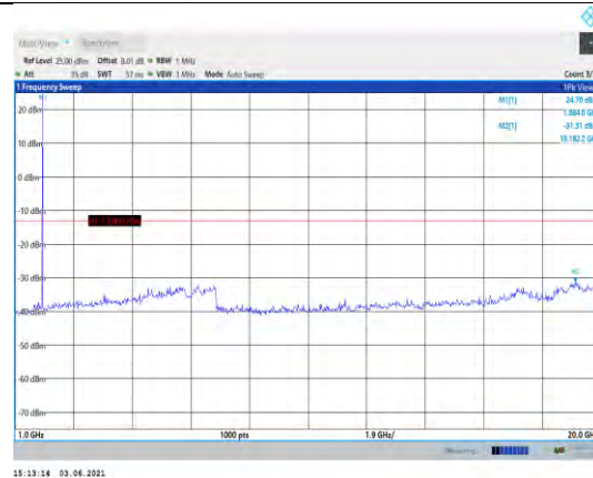
Band2-1.4MHz-16QAM-18900-1RB#0- Range2:1000~20000MHz
