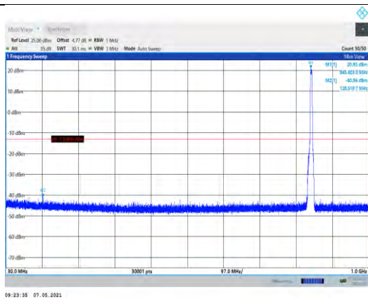
Band5-4233-30~1000MHz
