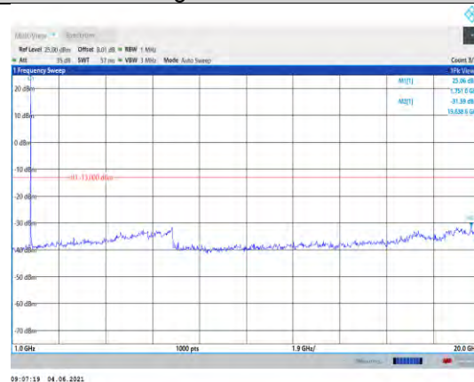
Band4-3MHz-16QAM-20385-1RB#0- Range2:1000~20000MHz
