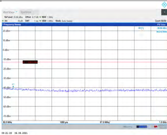
Band4-20MHz-16QAM-20050-1RB#0- Range1:30~1000MHz
