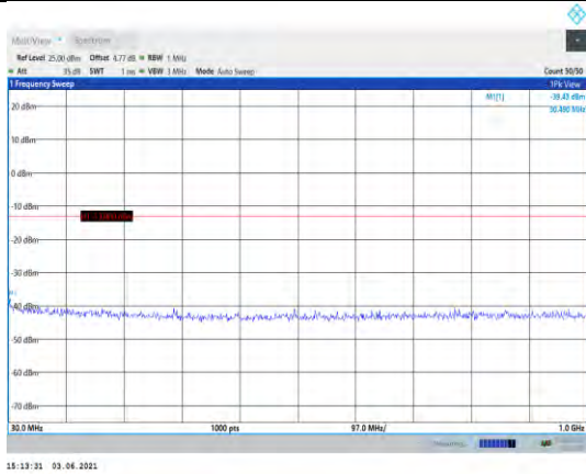
Band2-1.4MHz-QPSK-19193-1RB#0- Range1:30~1000MHz
