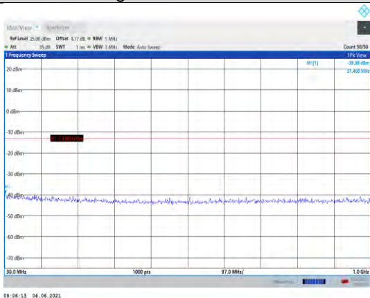
Band4-3MHz-16QAM-20175-1RB#0- Range1:30~1000MHz
