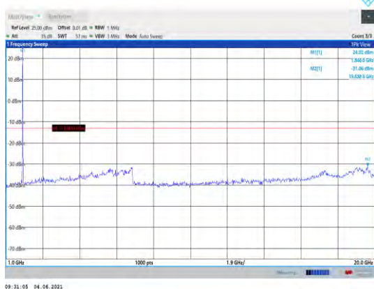
Band25-5MHz-16QAM-26065-1RB#0- Range2:1000~20000MHz
