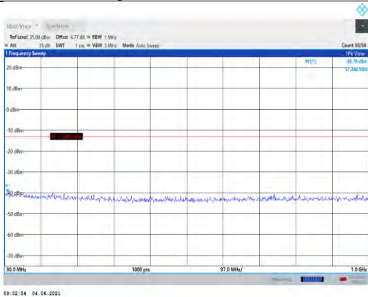
Band4-1.4MHz-16QAM-20175-1RB#0- Range1:30~1000MHz
