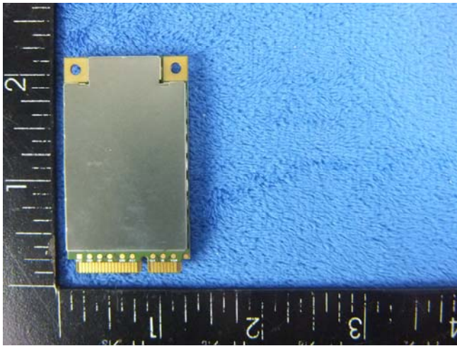
EUT – PCB 3 Rear View
