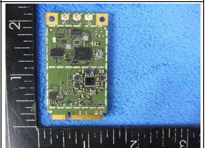
EUT - PCB 3 Front View
