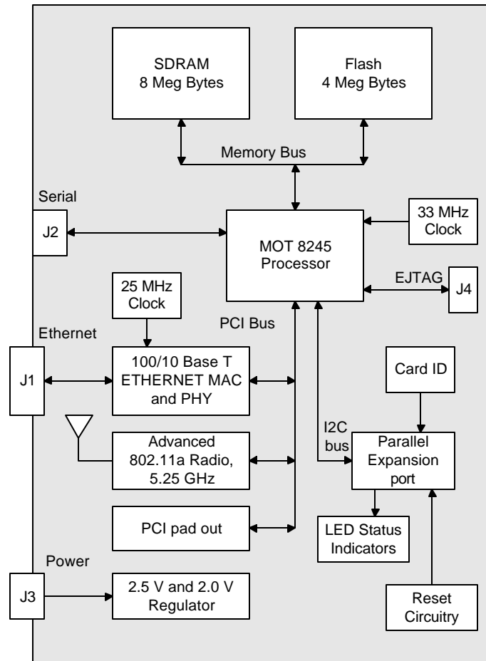
Model 2106 Block Diagram
