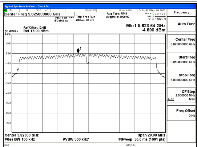
Mode:802.11n HT20 Frequency:5825MHz Ant:Chain1
