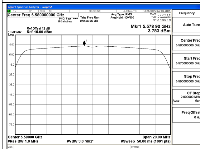
Mode:802.11ac VHT20 Frequency:5580MHz Ant:Chain1
