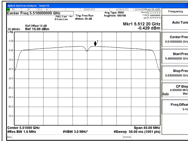
Mode:802.11n HT40 Frequency:5510MHz Ant:Chain0
