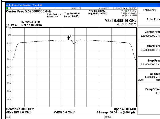
Mode:802.11n HT40 Frequency:5590MHz Ant:Chain1
