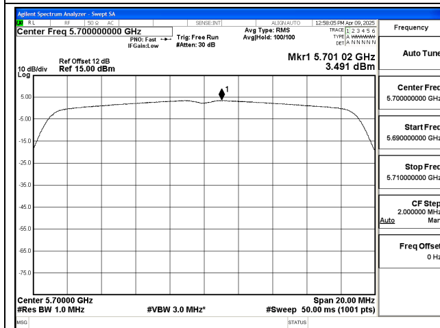
Mode:802.11ac VHT20 Frequency:5700MHz Ant:Chain0
