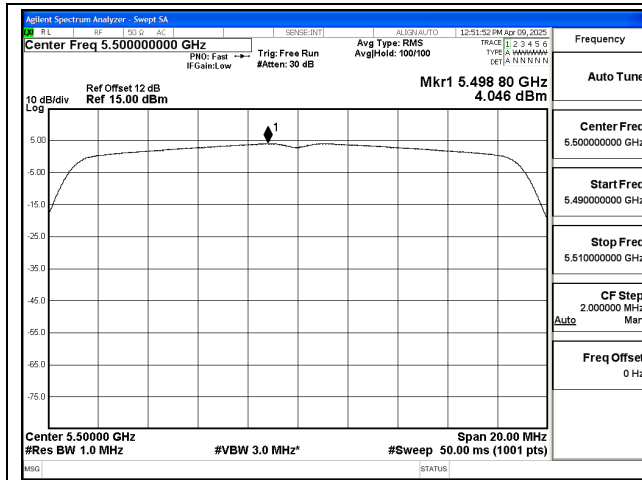
Mode:802.11ac VHT20 Frequency:5500MHz Ant:Chain0
