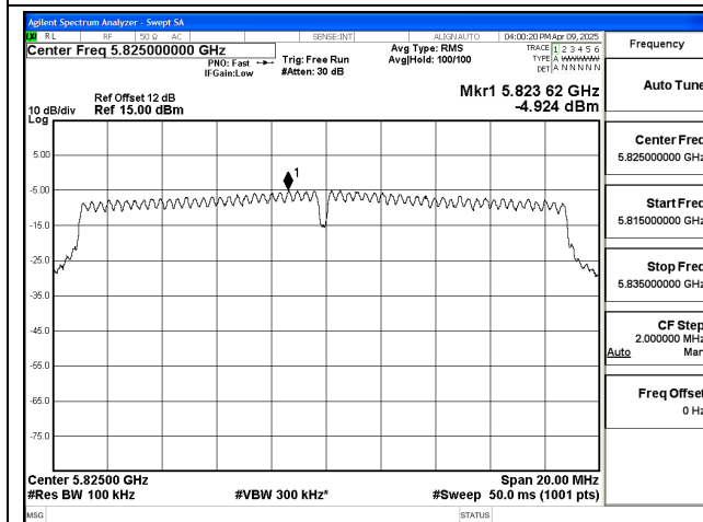
Mode:802.11n HT20 Frequency:5825MHz Ant:Chain0
