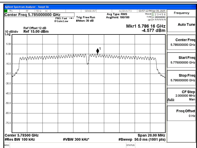
Mode:802.11n HT20 Frequency:5785MHz Ant:Chain0
