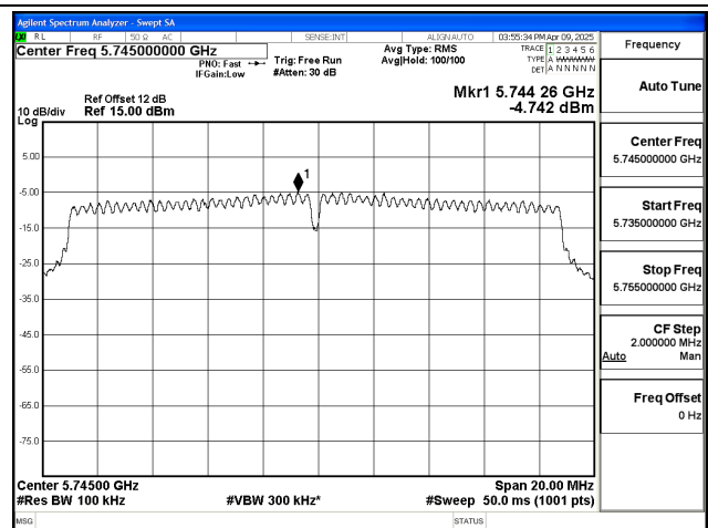
Mode:802.11n HT20 Frequency:5745MHz Ant:Chain1
