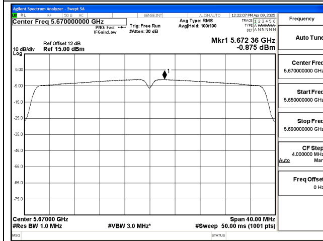
Mode:802.11n HT40 Frequency:5670MHz Ant:Chain0
