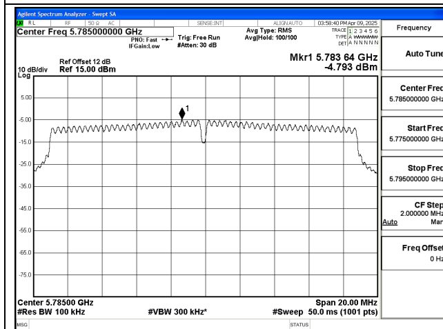
Mode:802.11n HT20 Frequency:5785MHz Ant:Chain1
