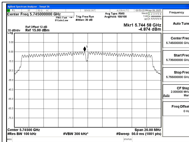
Mode:802.11n HT20 Frequency:5745MHz Ant:Chain0
