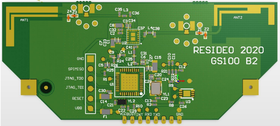
Figure 6 Daughter board bottom view
