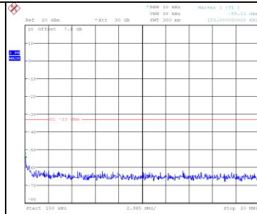
LTE Band 2_5MHz_CH18900 Spectrum Plot
