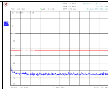
LTE Band 2_20MHz_CH18900 Spectrum Plot
