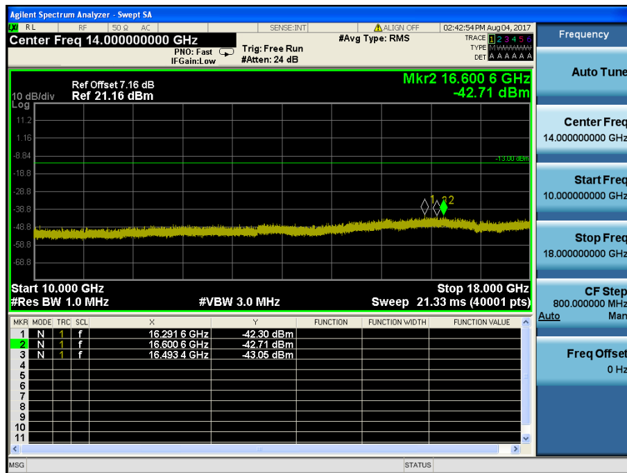
LTE Band 4 / 20MHz / 16QAM - RB Size/Offset (1/0)–Mid Channel
