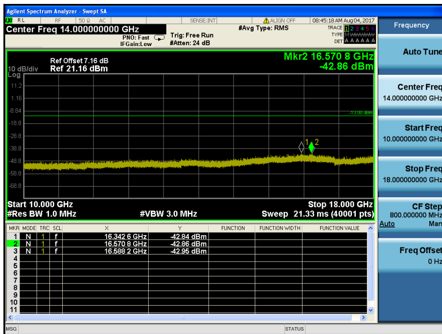
LTE Band 4 / 15MHz / QPSK - RB Size/Offset (1/37)–Low Channel
