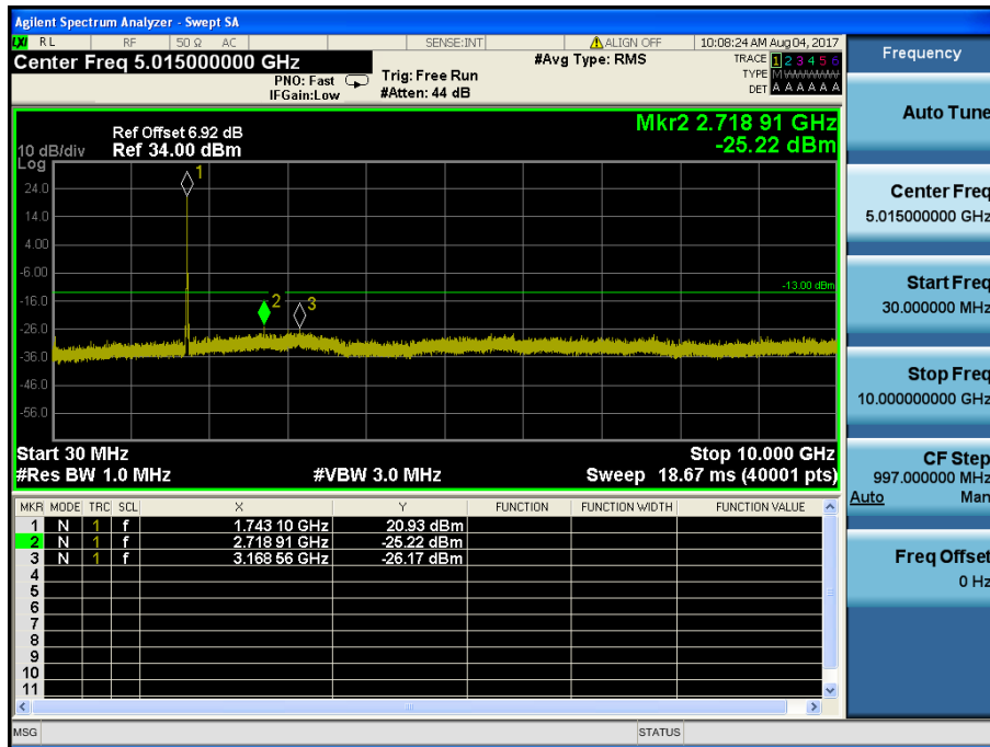
LTE Band 4 / 20MHz / QPSK - RB Size/Offset (50/0) – High Channel
