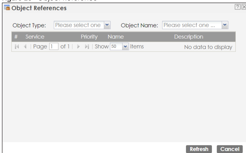
Figure 28 Object Reference
