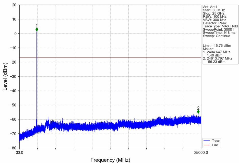
Zigbee_LCH_2405MHz_Ant1_NTNV
