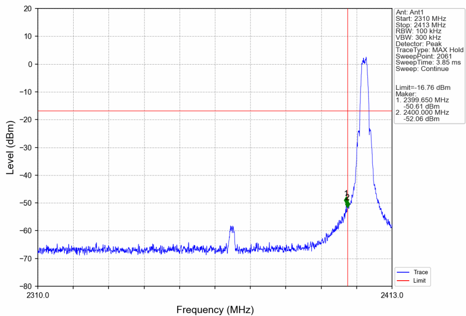
Zigbee_LCH_2405MHz_Ant1_NTNV
