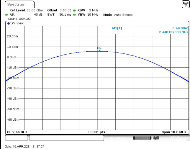
Channel 19 (2440MHz)
