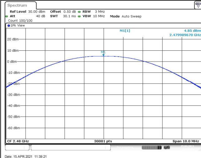
Channel 39 (2480MHz)
