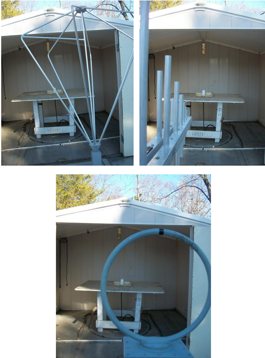
Figure 3.1 Radiated Test Setup
