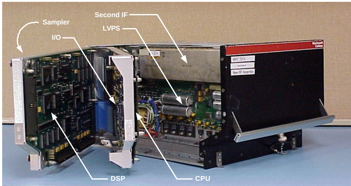
Figure C-7. WRT-701 Left Open
