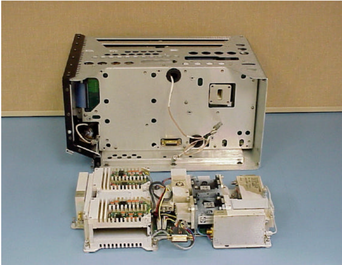
Figure C-8. RT Right Modules Removed
