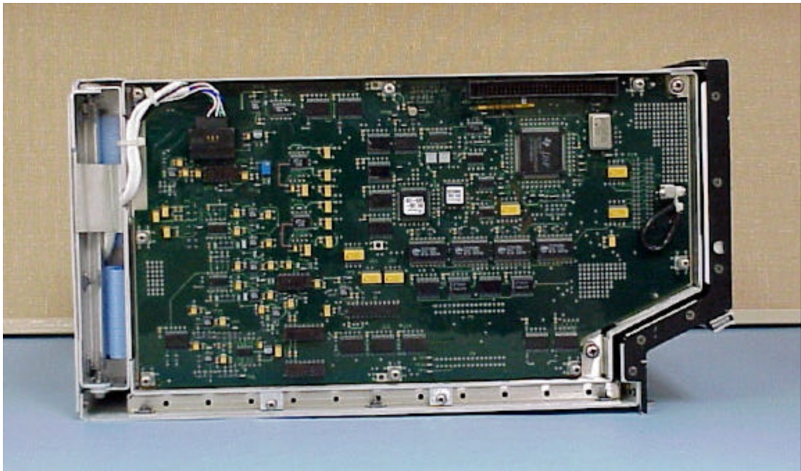
Figure C-5. WRT-701 Left Side
