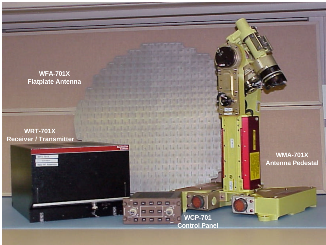
Figure C-1. WXR-701 Family
