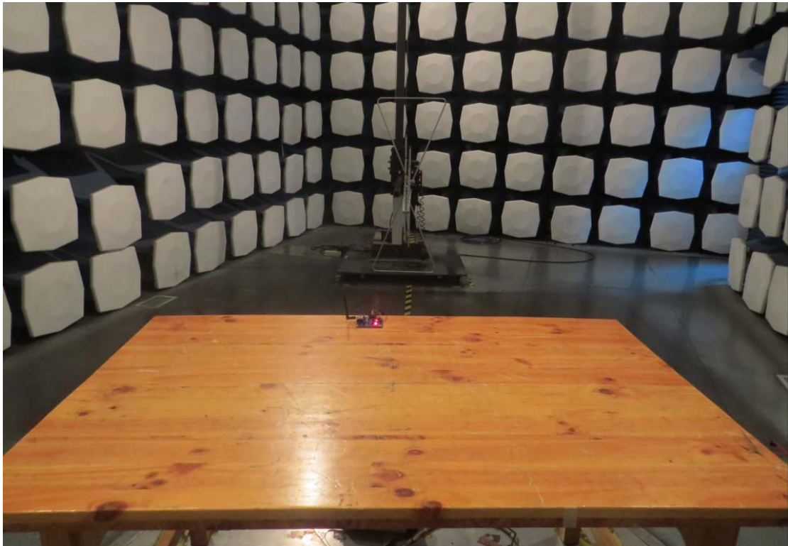
2AC7Z-ESP8266EX Test Setup photo
