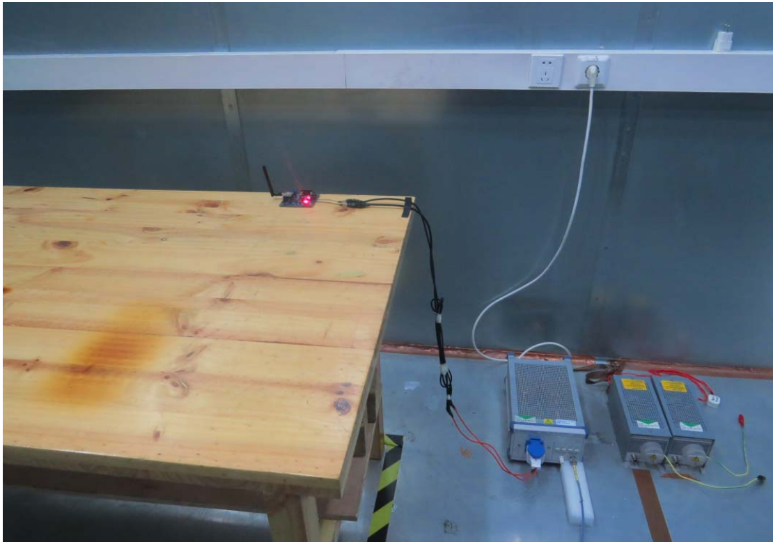
Conducted Emission Test Setup
