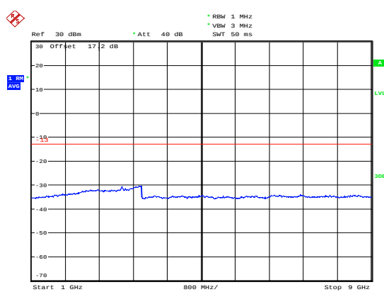
NB-IOT Band 5 CH-Middle 1GHz-9GHz
