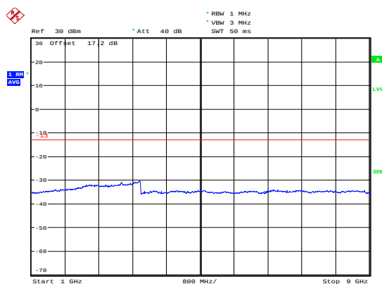
NB-IOT Band 5 CH-Low 1GHz-9GHz
