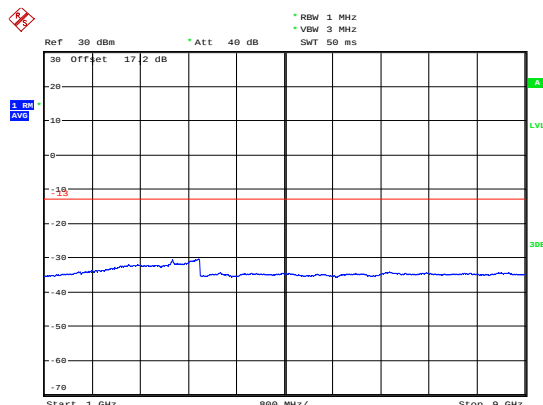
NB-IOT Band 5 CH-High 1GHz-9GHz
