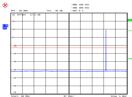
NB-IOT Band 5 CH-Low 30MHz-1GHz
