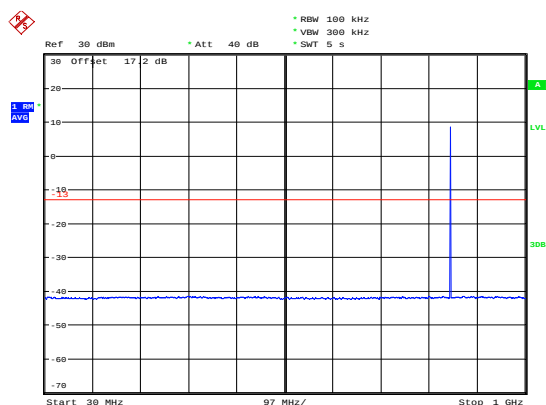
NB-IOT Band 5 CH-High 30MHz-1GHz
