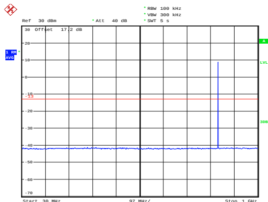
NB-IOT Band 5 CH-Middle 30MHz-1GHz
