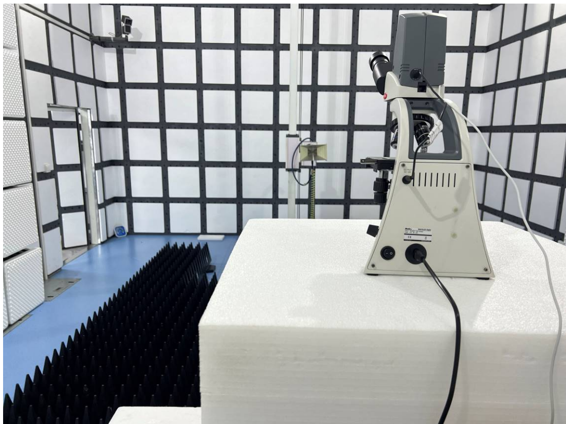
RE- Front View (3GHz-18GHz)
