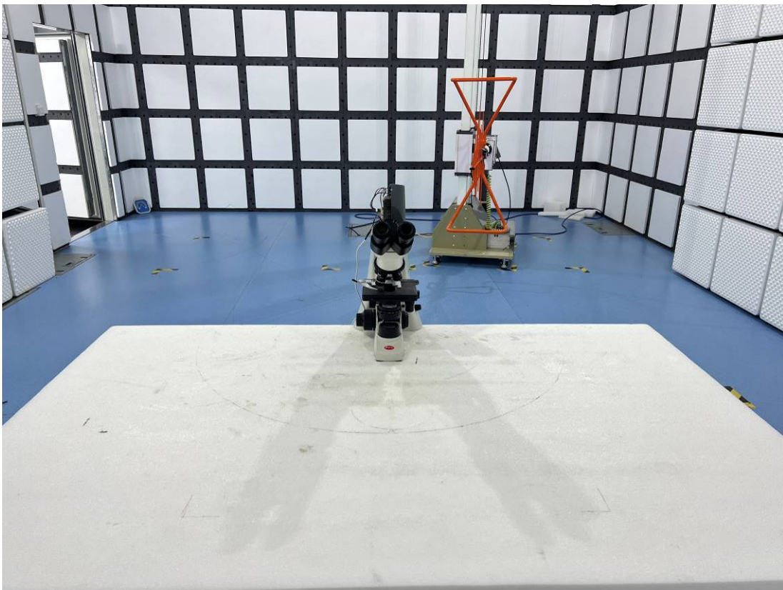
RE- Front View (Below 1GHz)
