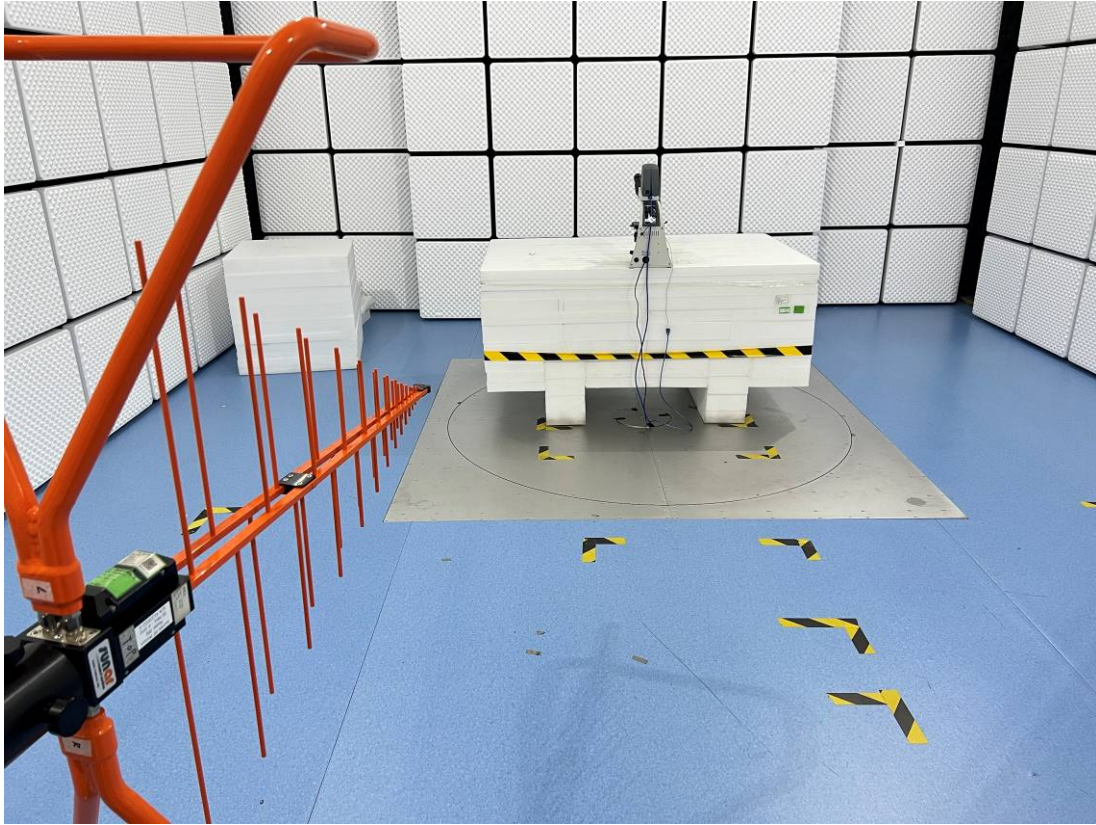
RE- Front View (1GHz-3GHz)
