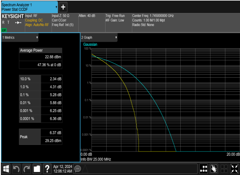
N66(20M)_DFT-s-OFDM_QPSK_Outer_Full_Mid_CH
