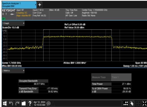
N66(40M)_CP-OFDM_16 QAM_Outer_Full_Mid_CH
