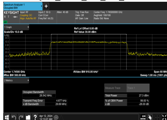
N66(30M)_CP-OFDM_16 QAM_Outer_Full_Mid_CH
