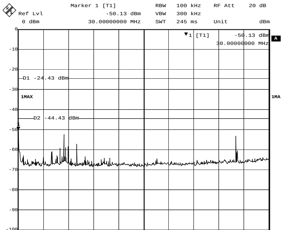
CH00 Data rate 1Mbps 30MHz to 1GHz
