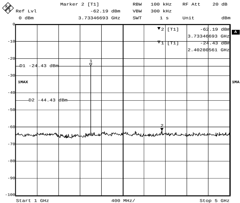
CH00 Data rate 1Mbps 1GHz to 5GHz
