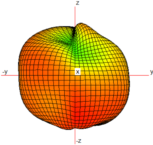
3D Antenna pattern
