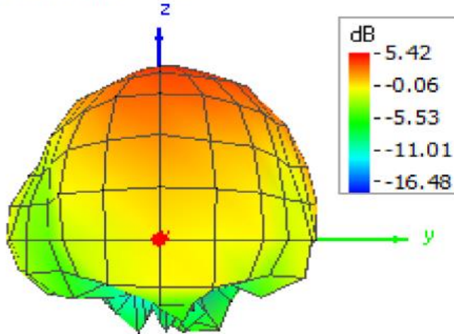
Figure F-2 Pattern at 5825 MHz (Front / Back view)
