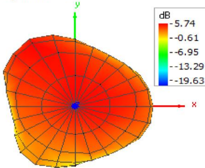
Figure E-1 Pattern at 5580 MHz (Top / Bottom view)
