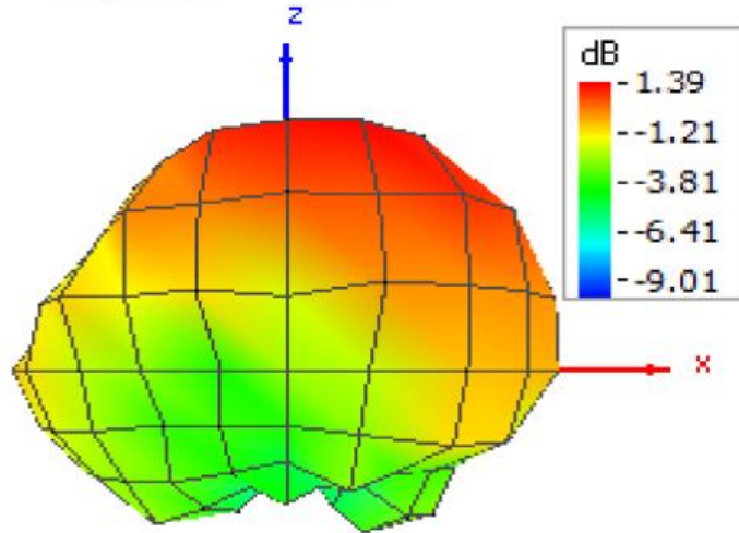
Figure C-3 Pattern at 2472 MHz (Left / Right view)
