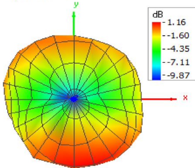
Figure B-1 Pattern at 2442 MHz (Top / Bottom view)
