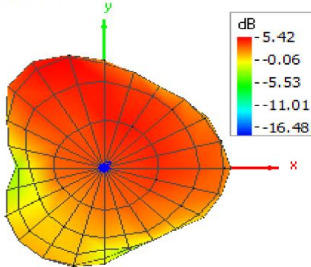
Figure F-1 Pattern at 5825 MHz (Top / Bottom view)
