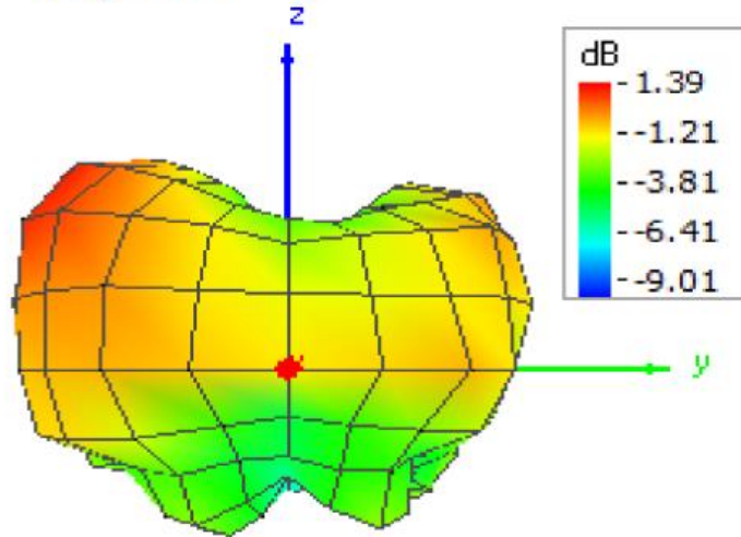
Figure C-2 Pattern at 2472 MHz (Front / Back view)
