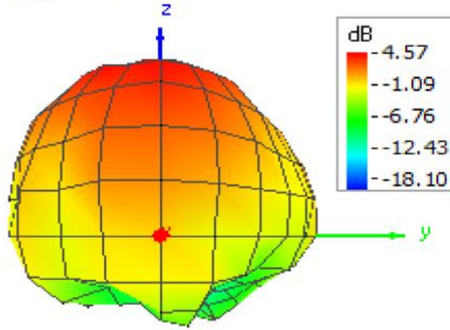
Figure D-2 Pattern at 5180 MHz (Front / Back view)
