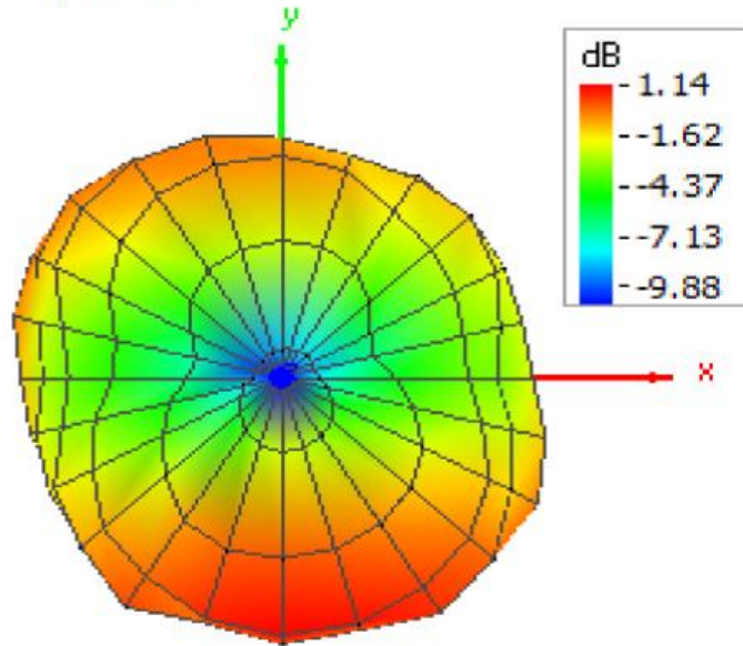
Figure A-1 Pattern at 2412 MHz (Top / Bottom view)
