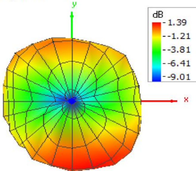
Figure C-1 Pattern at 2472 MHz (Top / Bottom view)
