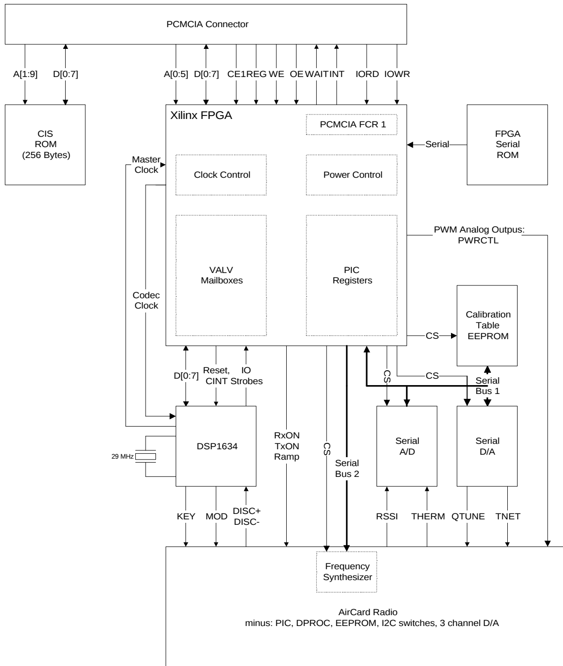
Figure 1: ACE Logic Block Diagram
