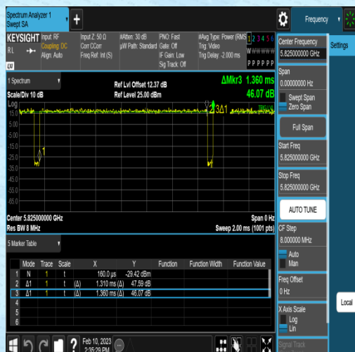
NTVN-11AC20SISO-Ant2-5825-1.31-1.36
