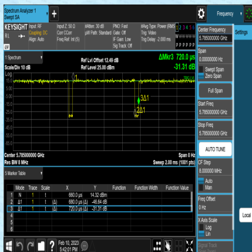
NTNV-11AC20MIMO-Ant1-5785-0.68-0.72
