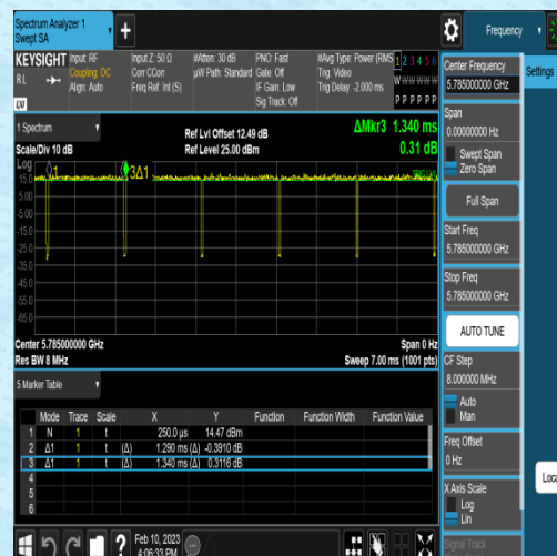
NTVN-11N20MIMO-Ant2-5785-1.29-1.34
