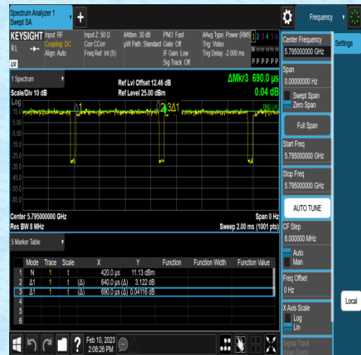
NTNV-11N40SISO-Ant2-5795-0.64-0.69
