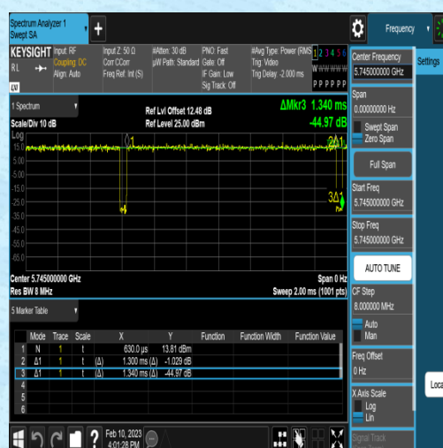
NTVN-11N20MIMO-Ant2-5745-1.30-1.34
