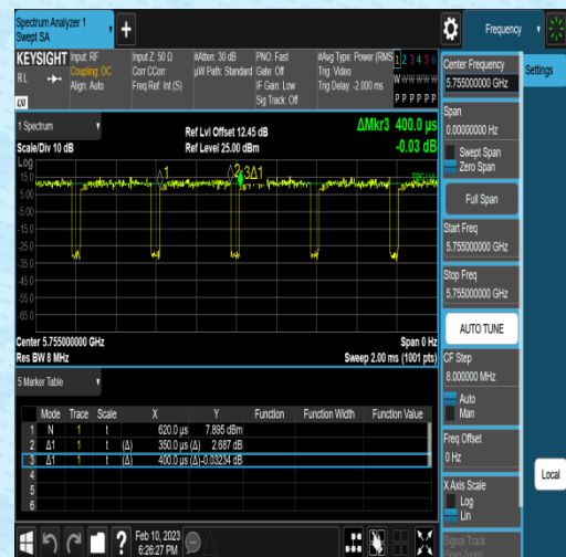
NTNV-11AC40MIMO-Ant2-5755-0.35-0.40
