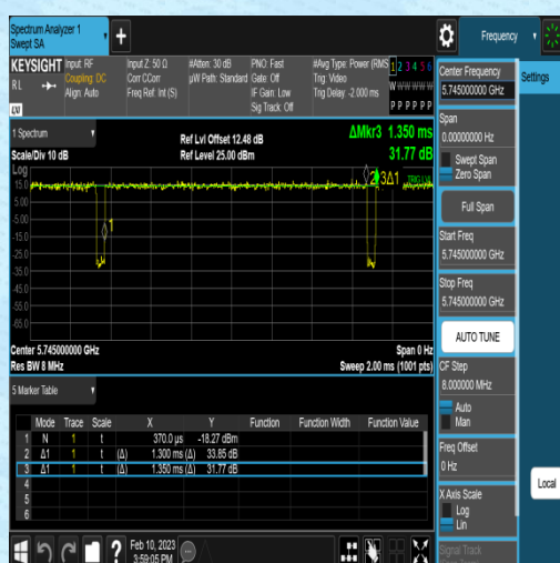
NTVN-11N20MIMO-Ant1-5745-1.30-1.35
