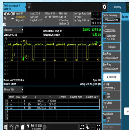
NTNV-11AC80MIMO-Ant2-5775-0.19-0.23
