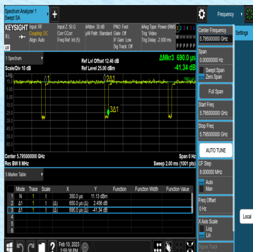
NTVN-11AC40SISO-Ant2-5795-0.65-0.69
