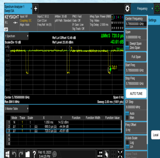
NTNV-11AC20MIMO-Ant2-5785-0.68-0.72
