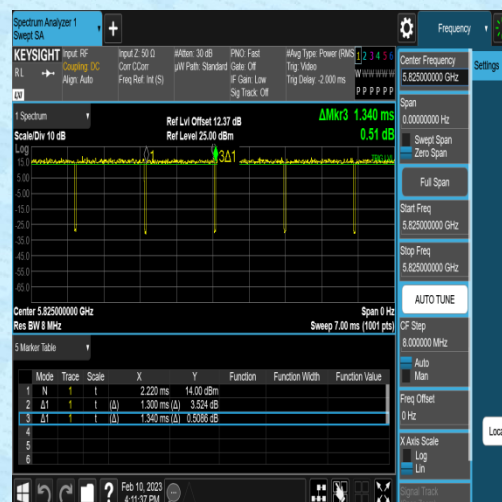
NTVN-11N20MIMO-Ant2-5825-1.30-1.34
