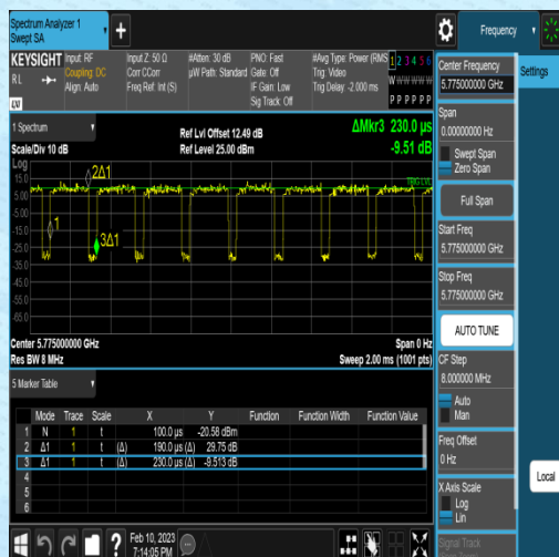
NTNV-11AC80MIMO-Ant1-5775-0.19-0.23
