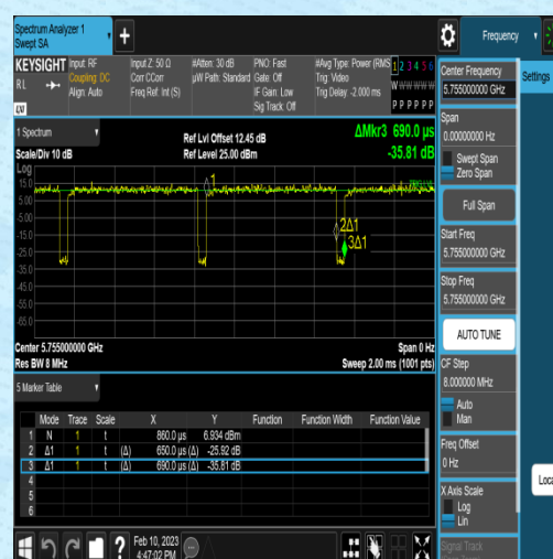
NTVN-11N40MIMO-Ant2-5755-0.65-0.69
