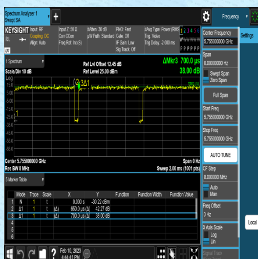
NTVN-11N40MIMO-Ant1-5755-0.65-0.70
