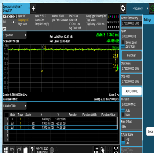
NTVN-11N20MIMO-Ant1-5785-1.30-1.34
