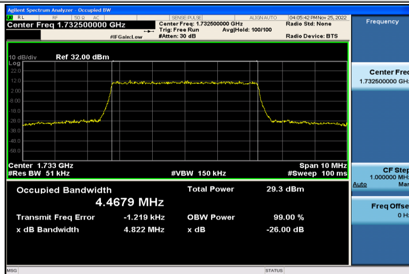
Band4-5MHz-64QAM-20175-25RB#0-4.4679
