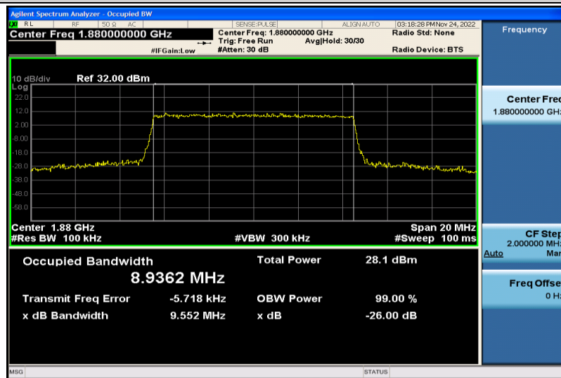
Band2-10MHz-16QAM-18900-50RB#0-8.9362
