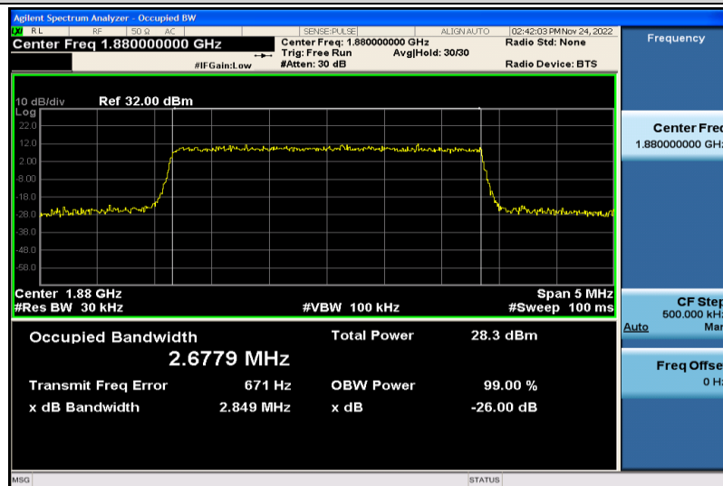
Band2-3MHz-QPSK-18900-15RB#0-2.6779
