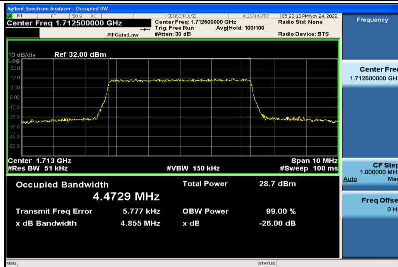
Band4-5MHz-16QAM-19975-25RB#0-4.4729
