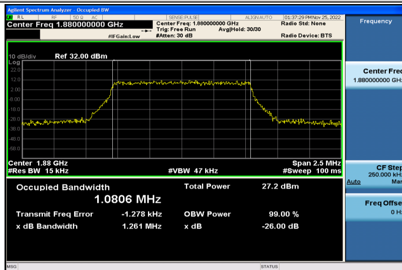
Band2-1.4MHz-64QAM-18900-6RB#0-1.0806
