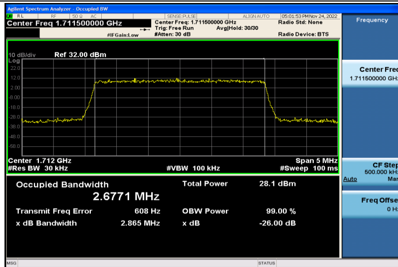
Band4-3MHz-16QAM-19965-15RB#0-2.6771
