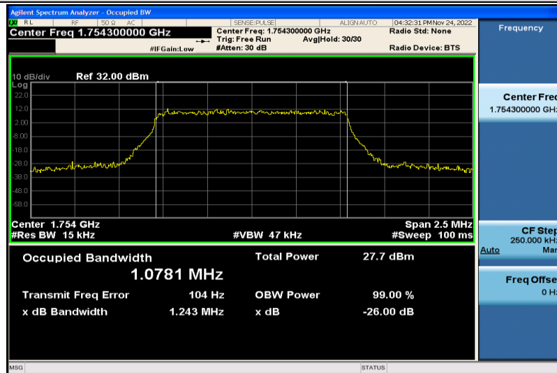
Band4-1.4MHz-16QAM-20393-6RB#0-1.0781
