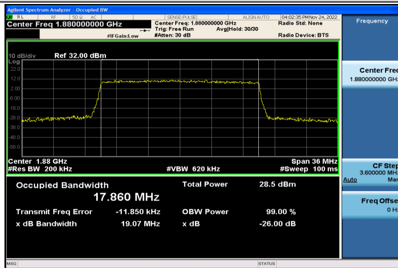
Band2-20MHz-16QAM-18900-100RB#0-17.860
