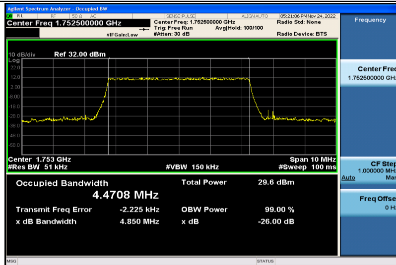
Band4-5MHz-QPSK-20375-25RB#0-4.4708
