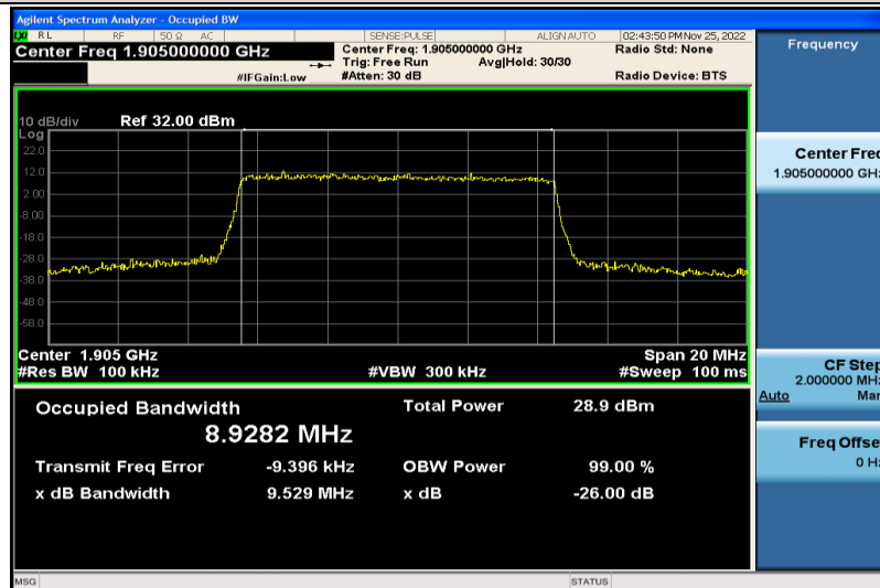
Band2-10MHz-64QAM-19150-50RB#0-8.9282
