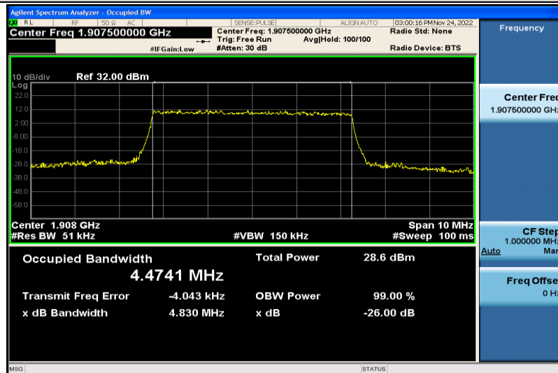
Band2-5MHz-QPSK-19175-25RB#0-4.4741
