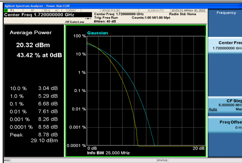
Band66-20MHz-64QAM-132072-100RB#0
