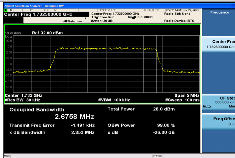
Band4-3MHz-16QAM-20175-15RB#0-2.6758
