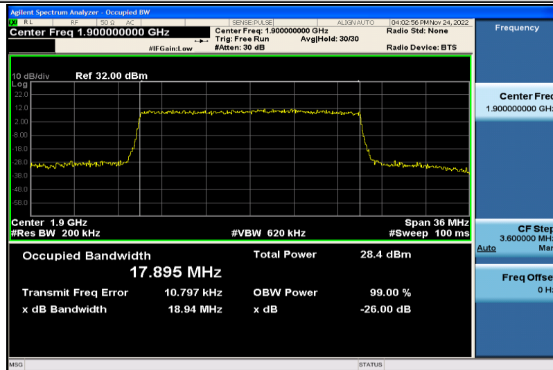
Band2-20MHz-16QAM-19100-100RB#0-17.895
