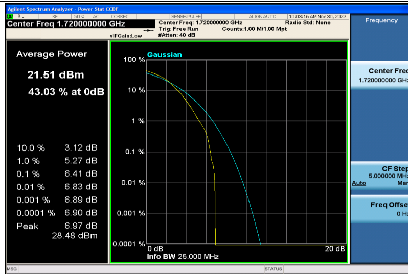
Band66-20MHz-64QAM-132072-1RB#0
