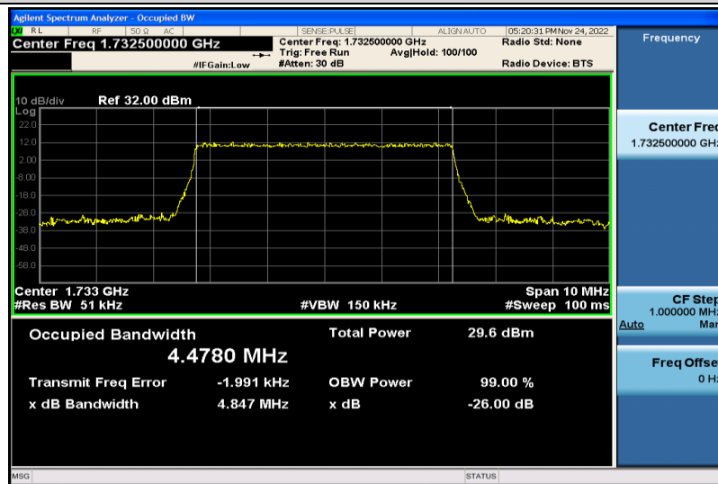
Band4-5MHz-QPSK-20175-25RB#0-4.4780
