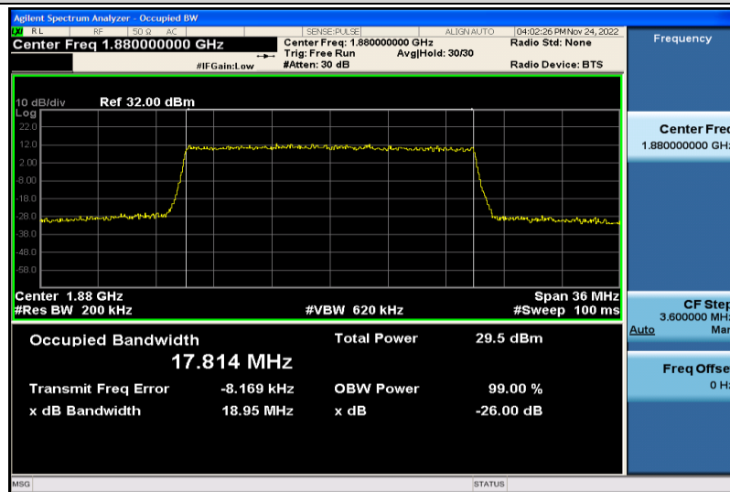
Band2-20MHz-QPSK-18900-100RB#0-17.814
