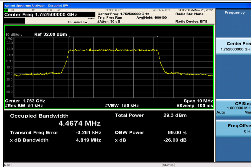
Band4-5MHz-64QAM-20375-25RB#0-4.4674
