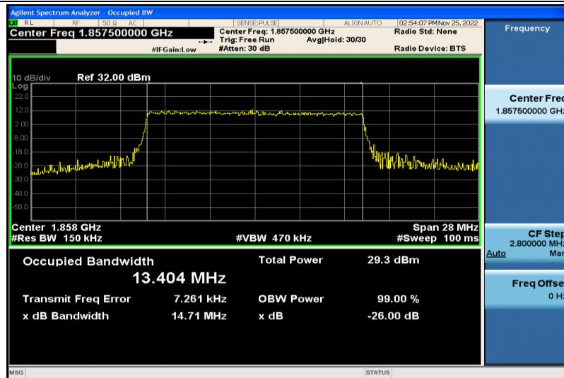
Band2-15MHz-64QAM-18675-75RB#0-13.404
