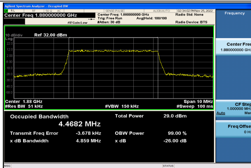
Band2-5MHz-64QAM-18900-25RB#0-4.4682
