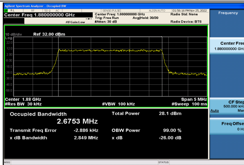
Band2-3MHz-64QAM-18900-15RB#0-2.6753
