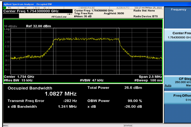
Band4-1.4MHz-64QAM-20393-6RB#0-1.0827
