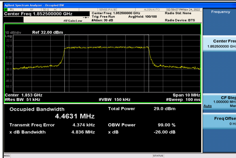
Band2-5MHz-QPSK-18625-25RB#0-4.4631
