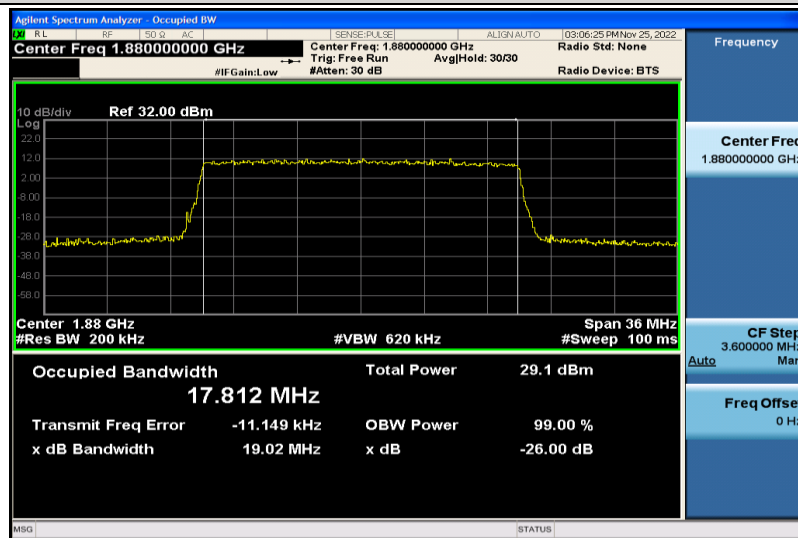
Band2-20MHz-64QAM-18900-100RB#0-17.812
