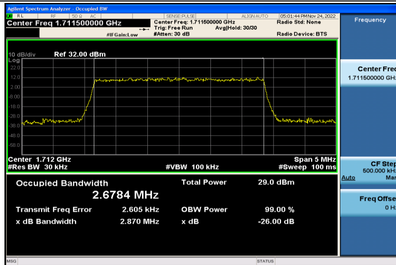
Band4-3MHz-QPSK-19965-15RB#0-2.6784
