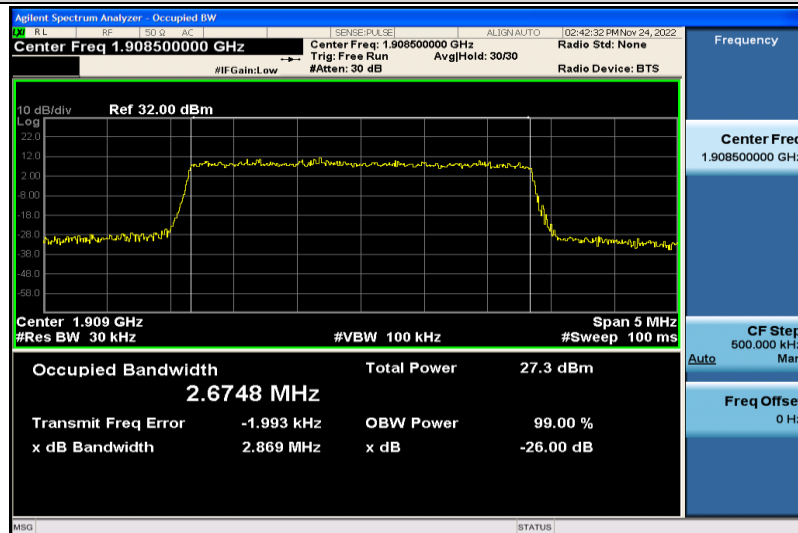
Band2-3MHz-16QAM-19185-15RB#0-2.6748
