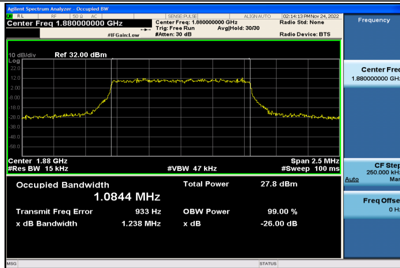
Band2-1.4MHz-QPSK-18900-6RB#0-1.0844
