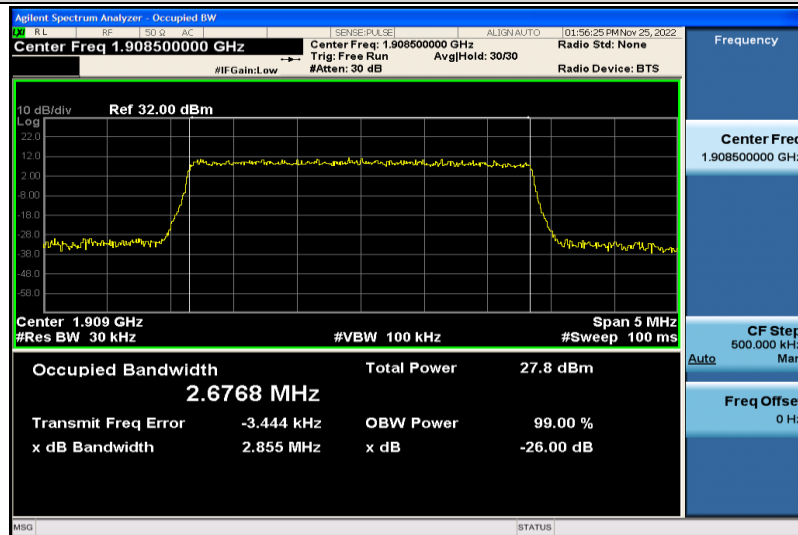
Band2-3MHz-64QAM-19185-15RB#0-2.6768
