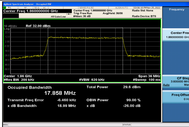
Band2-20MHz-64QAM-18700-100RB#0-17.858
