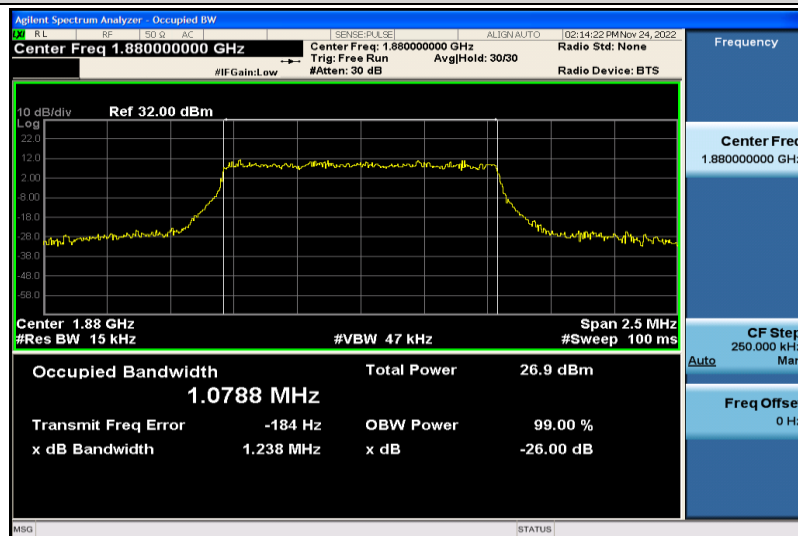
Band2-1.4MHz-16QAM-18900-6RB#0-1.0788
