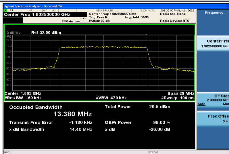
Band2-15MHz-QPSK-19125-75RB#0-13.380
