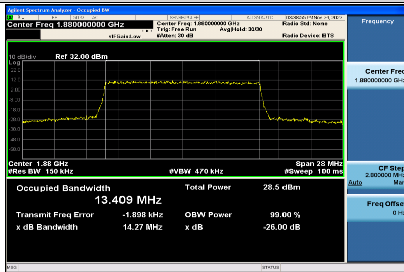
Band2-15MHz-16QAM-18900-75RB#0-13.409
