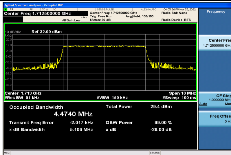
Band4-5MHz-64QAM-19975-25RB#0-4.4740
