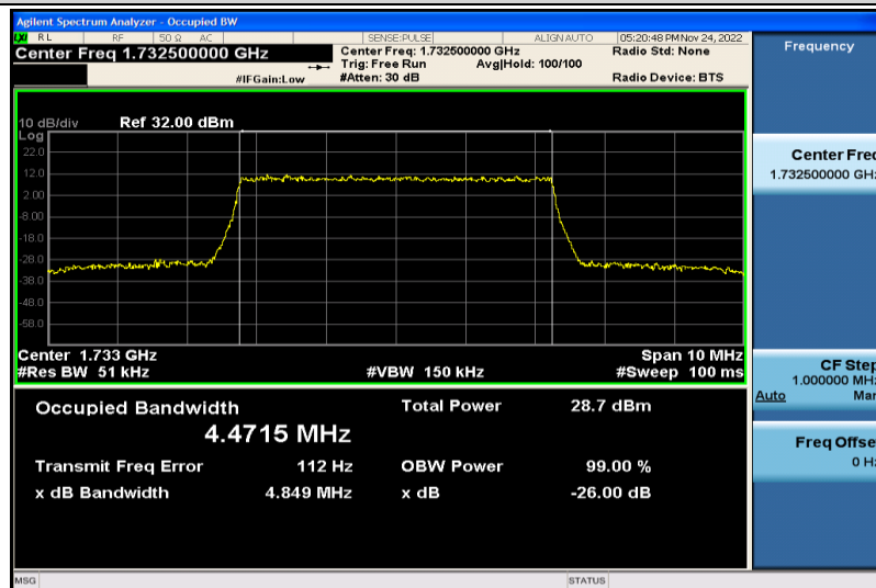
Band4-5MHz-16QAM-20175-25RB#0-4.4715
