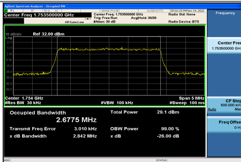
Band4-3MHz-QPSK-20385-15RB#0-2.6775
