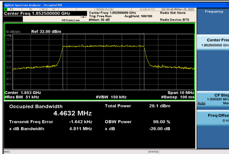
Band2-5MHz-64QAM-18625-25RB#0-4.4632
