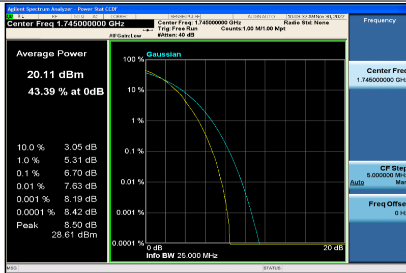
Band66-20MHz-64QAM-132322-100RB#0
