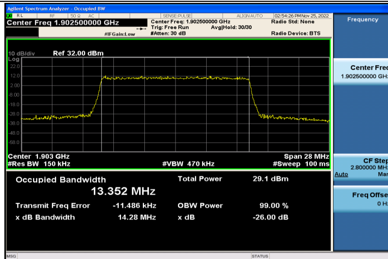
Band2-15MHz-64QAM-19125-75RB#0-13.352
