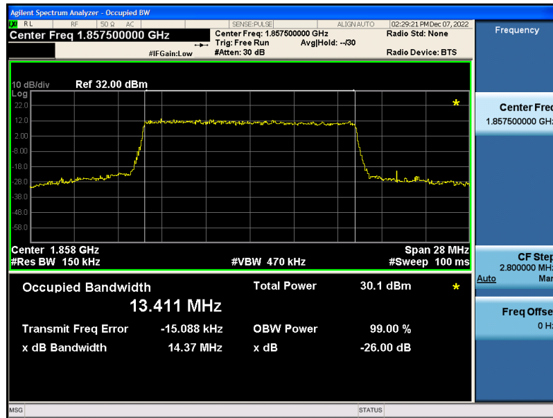
Band2-15MHz-QPSK-18675-75RB#0-13.411
