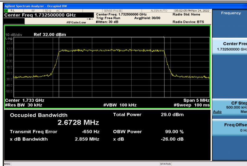
Band4-3MHz-QPSK-20175-15RB#0-2.6728
