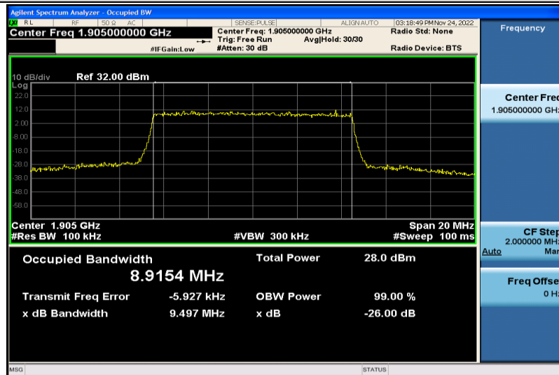
Band2-10MHz-16QAM-19150-50RB#0-8.9154
