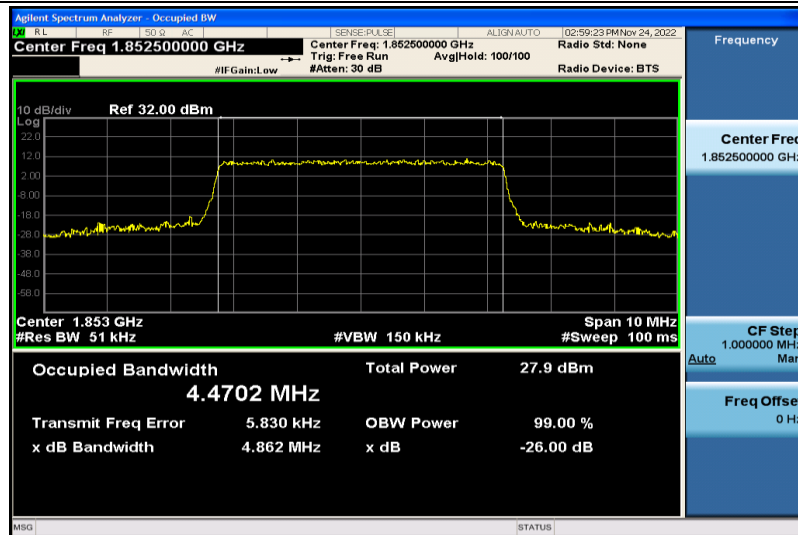
Band2-5MHz-16QAM-18625-25RB#0-4.4702
