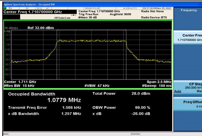
Band4-1.4MHz-64QAM-19957-6RB#0-1.0779
