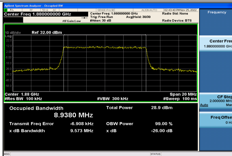
Band2-10MHz-64QAM-18900-50RB#0-8.9380
