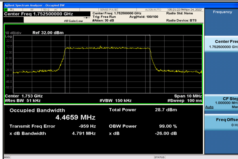
Band4-5MHz-16QAM-20375-25RB#0-4.4659
