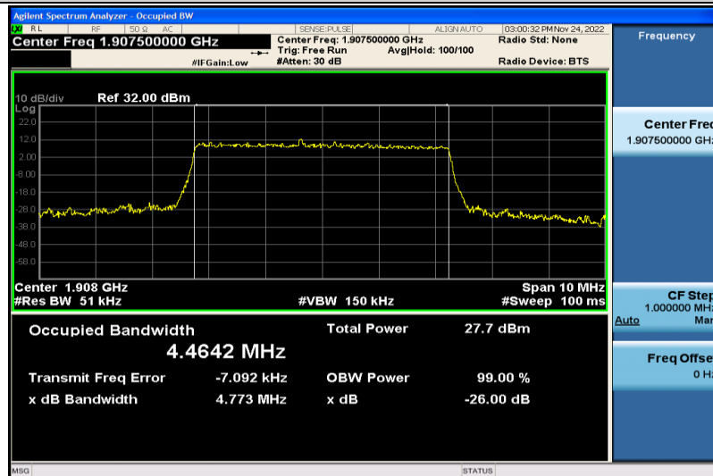
Band2-5MHz-16QAM-19175-25RB#0-4.4642
