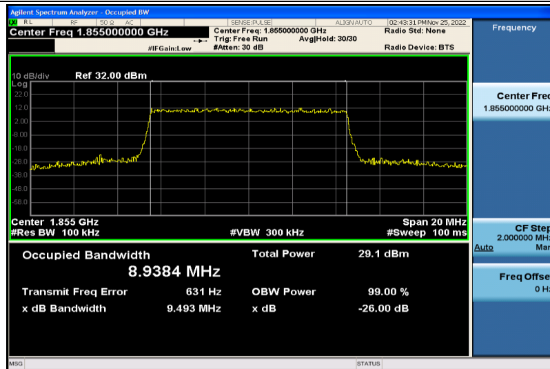
Band2-10MHz-64QAM-18650-50RB#0-8.9384
