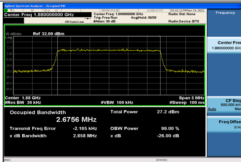
Band2-3MHz-16QAM-18900-15RB#0-2.6756
