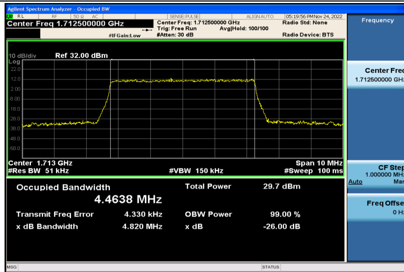
Band4-5MHz-QPSK-19975-25RB#0-4.4638
