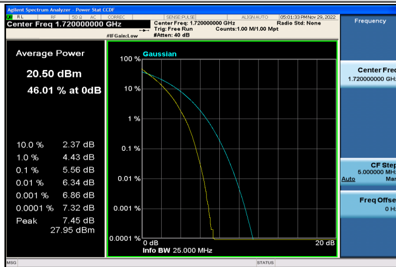
Band66-20MHz-QPSK-132072-100RB#0
