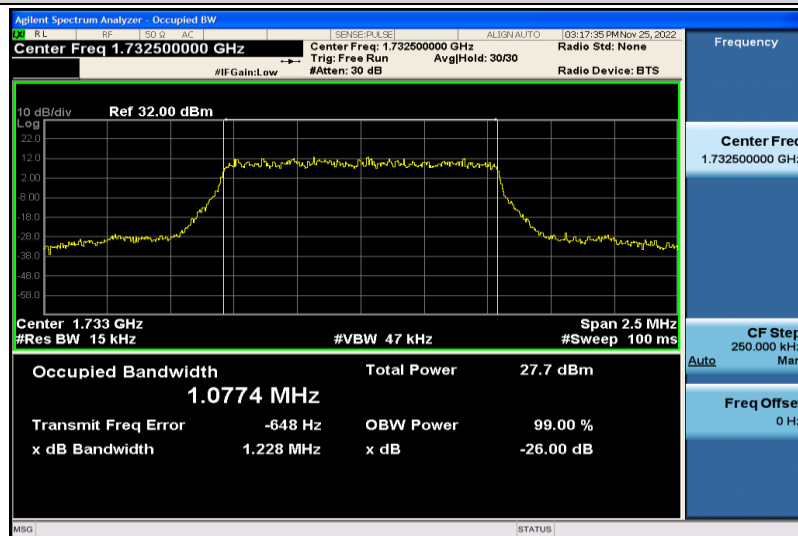
Band4-1.4MHz-64QAM-20175-6RB#0-1.0774
