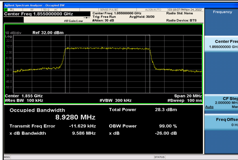
Band2-10MHz-16QAM-18650-50RB#0-8.9280
