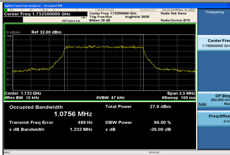
Band4-1.4MHz-16QAM-20175-6RB#0-1.0756
