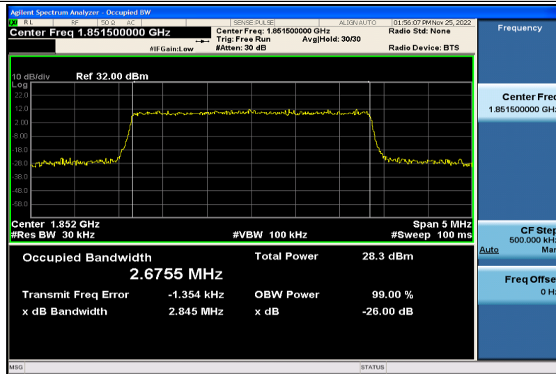
Band2-3MHz-64QAM-18615-15RB#0-2.6755
