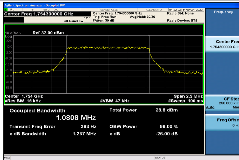
Band4-1.4MHz-QPSK-20393-6RB#0-1.0808
