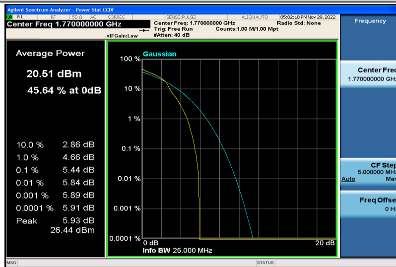
Band66-20MHz-16QAM-132572-1RB#0
