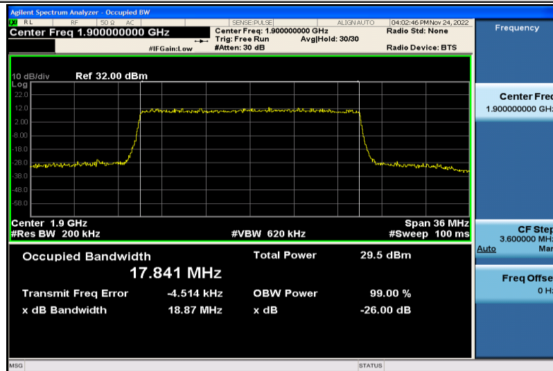
Band2-20MHz-QPSK-19100-100RB#0-17.841
