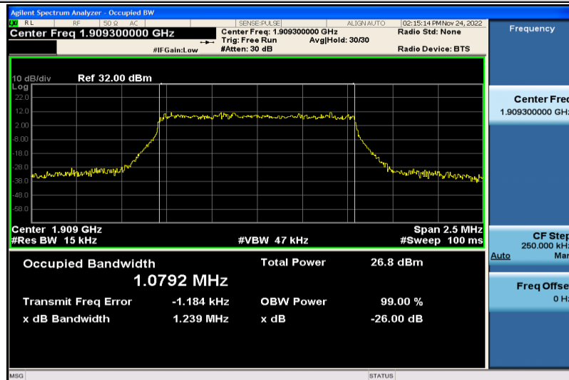
Band2-1.4MHz-16QAM-19193-6RB#0-1.0792
