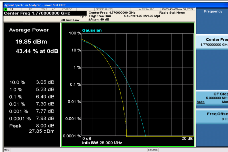
Band66-20MHz-64QAM-132572-100RB#0
