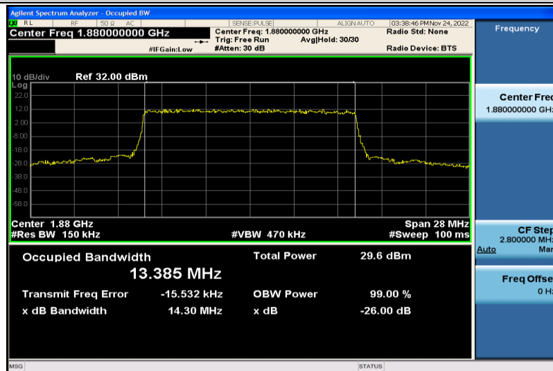
Band2-15MHz-QPSK-18900-75RB#0-13.385
