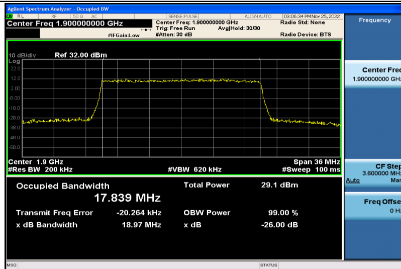
Band2-20MHz-64QAM-19100-100RB#0-17.839
