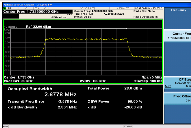
Band4-3MHz-64QAM-20175-15RB#0-2.6778
