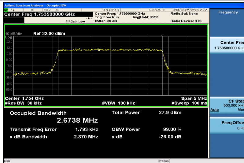
Band4-3MHz-16QAM-20385-15RB#0-2.6738
