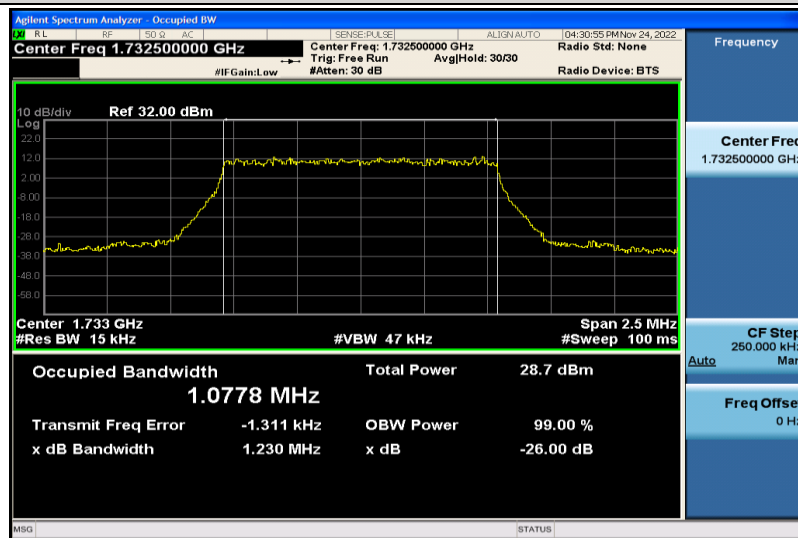
Band4-1.4MHz-QPSK-20175-6RB#0-1.0778
