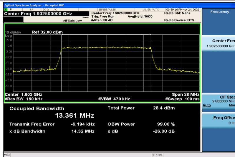
Band2-15MHz-16QAM-19125-75RB#0-13.361
