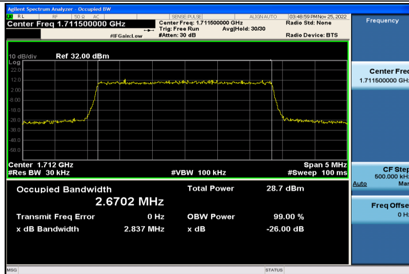
Band4-3MHz-64QAM-19965-15RB#0-2.6702
