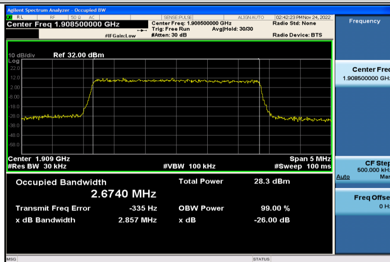
Band2-3MHz-QPSK-19185-15RB#0-2.6740
