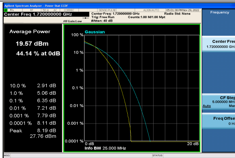
Band66-20MHz-16QAM-132072-100RB#0
