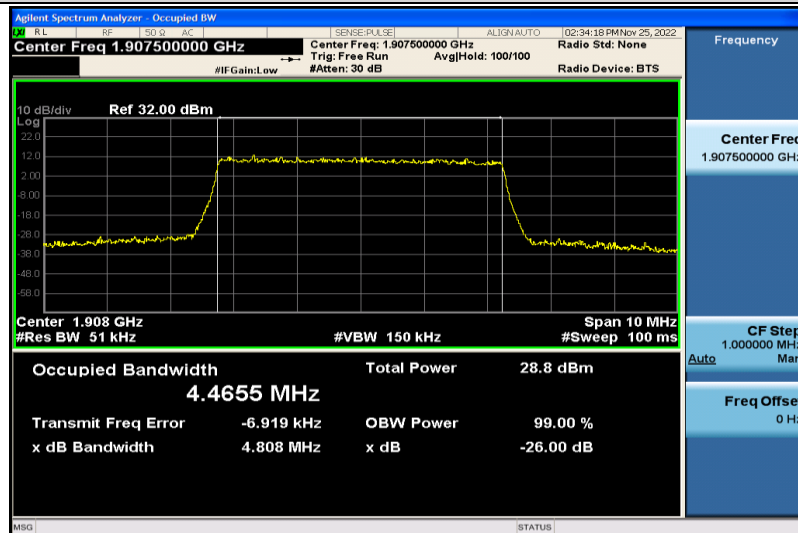
Band2-5MHz-64QAM-19175-25RB#0-4.4655
