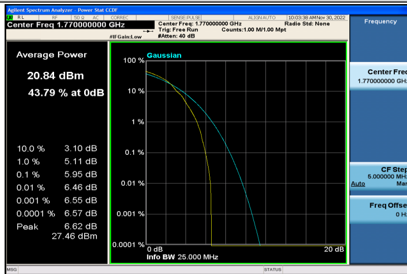
Band66-20MHz-64QAM-132572-1RB#0
