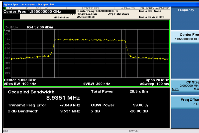
Band2-10MHz-QPSK-18650-50RB#0-8.9351
