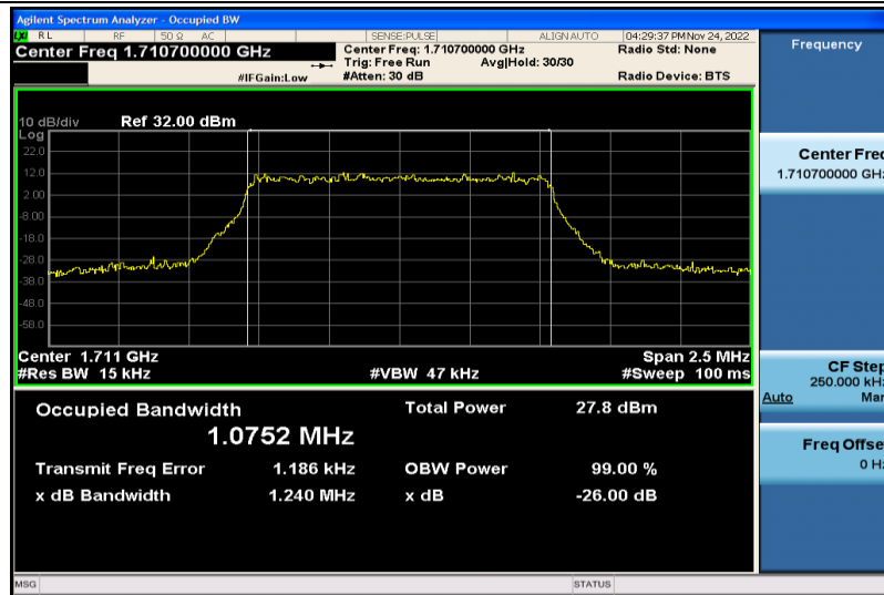
Band4-1.4MHz-16QAM-19957-6RB#0-1.0752
