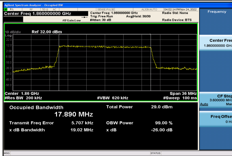
Band2-20MHz-16QAM-18700-100RB#0-17.890
