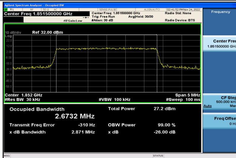
Band2-3MHz-16QAM-18615-15RB#0-2.6732
