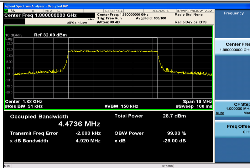
Band2-5MHz-QPSK-18900-25RB#0-4.4736
