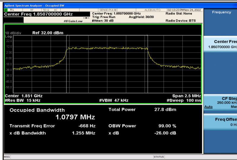
Band2-1.4MHz-QPSK-18607-6RB#0-1.0797
