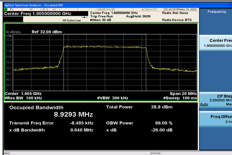
Band2-10MHz-QPSK-19150-50RB#0-8.9293
