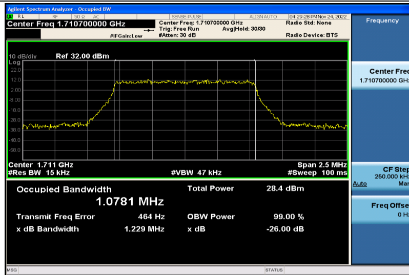
Band4-1.4MHz-QPSK-19957-6RB#0-1.0781
