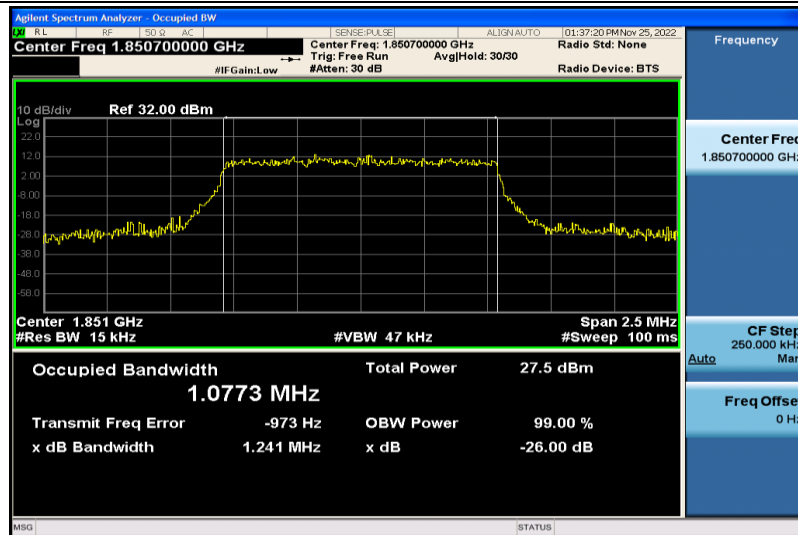
Band2-1.4MHz-64QAM-18607-6RB#0-1.0773
