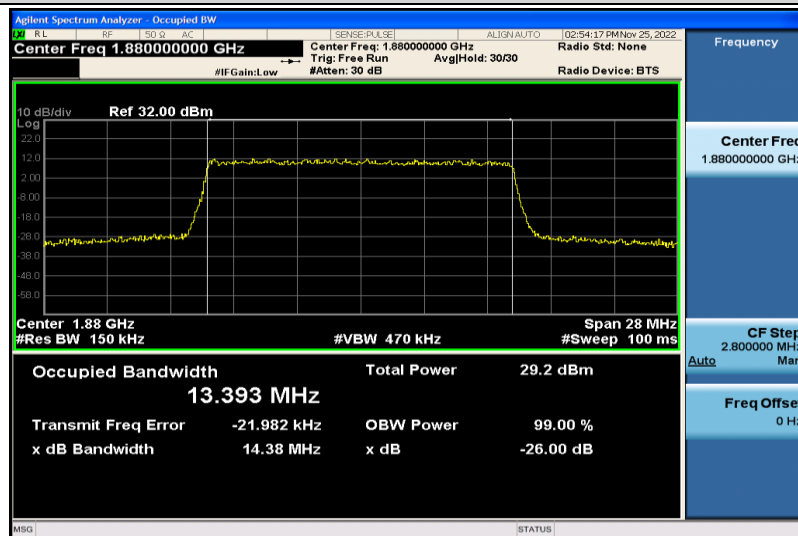
Band2-15MHz-64QAM-18900-75RB#0-13.393
