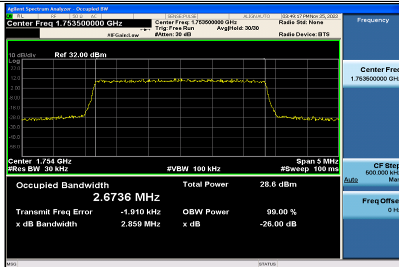
Band4-3MHz-64QAM-20385-15RB#0-2.6736
