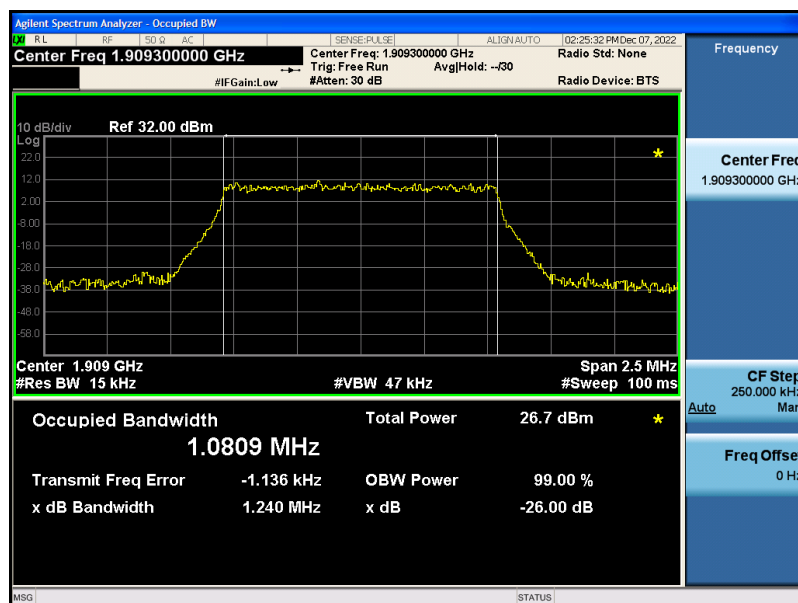
Band2-1.4MHz-64QAM-19193-6RB#0-1.0809
