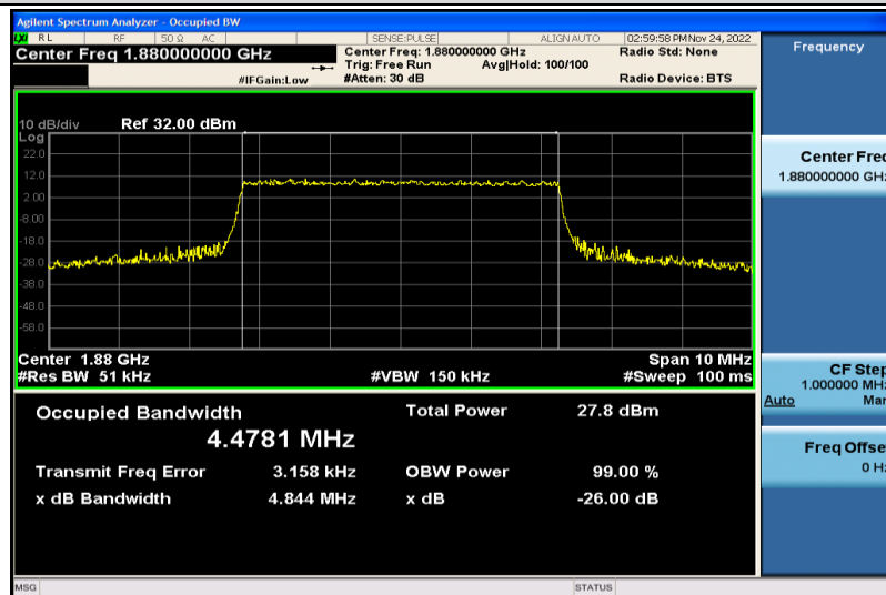
Band2-5MHz-16QAM-18900-25RB#0-4.4781
