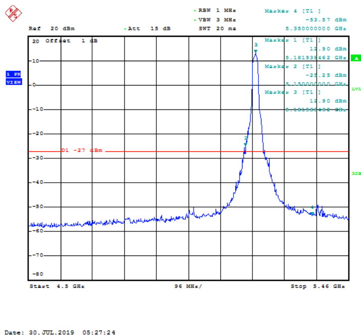
Fig. 19 Band Edges (802.11a, 5180MHz)
