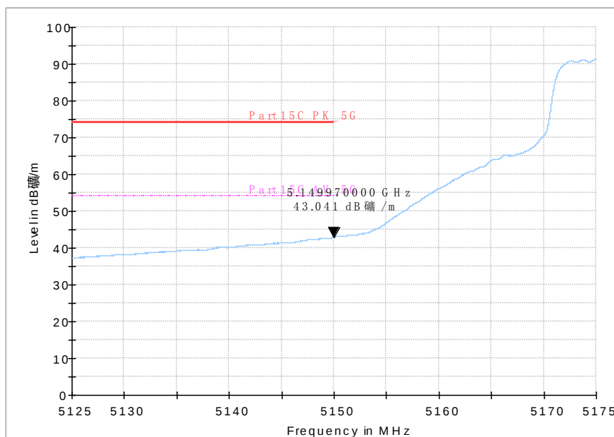
Fig. 27 Band Edges (802.11n-HT20, 5180MHz)
