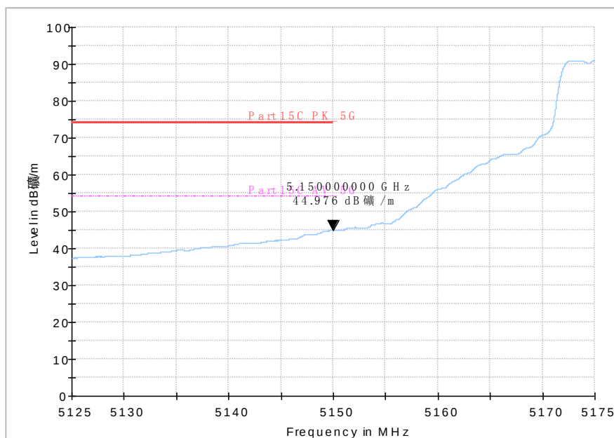
Fig. 25 Band Edges (802.11a, 5180MHz)
