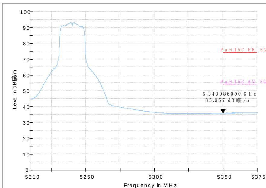
Fig. 28 Band Edges (802.11n-HT20, 5240MHz)
