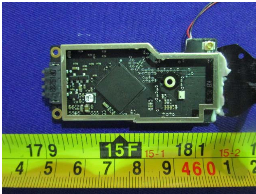
EUT –Board 4 Bottom Uncover View
