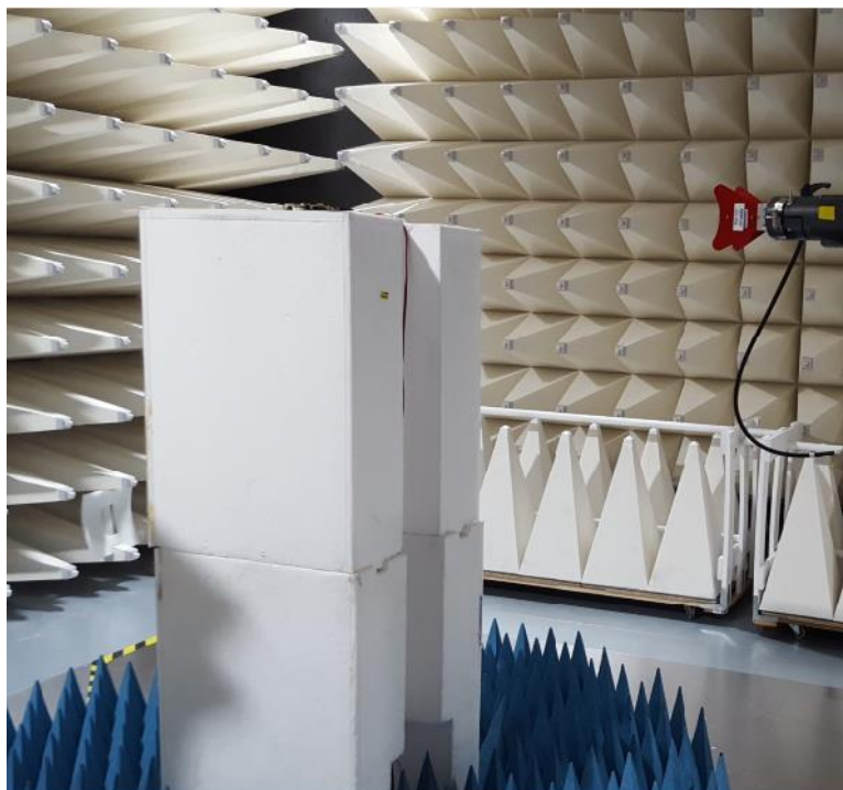
Figure F5. Radiated Setup 2
