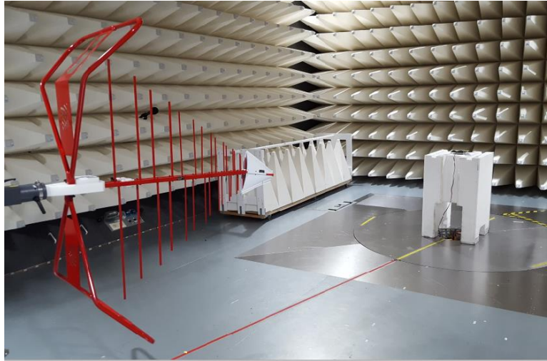
Figure F4. Radiated Setup 1
