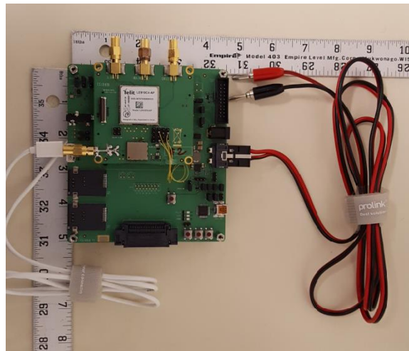
Figure F1: Conducted DUT top view with board and module
