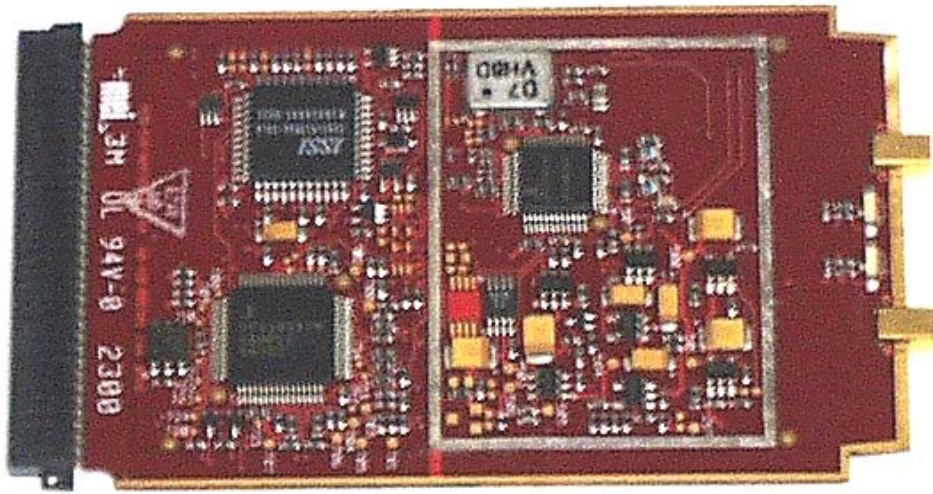
WLAN PCB Top view
