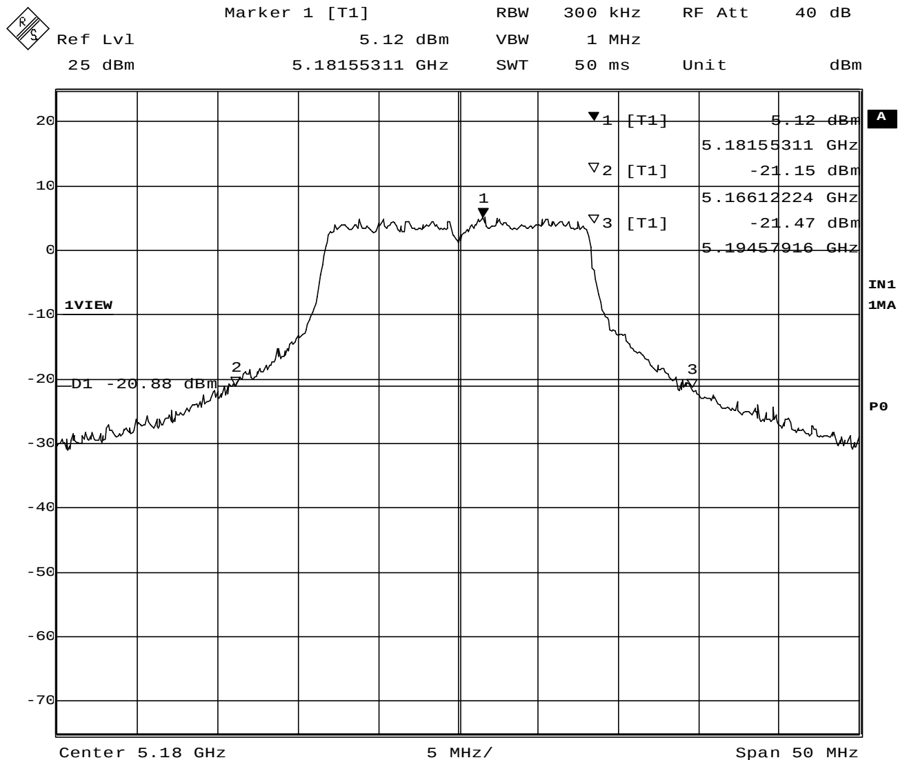
Plot 1-1. 26dB BW at 5180MHz
