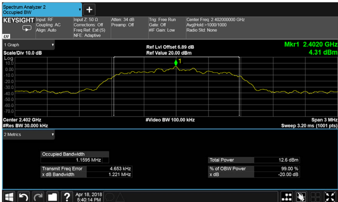
Figure 16 – 2402 MHz - 8-DPSK
