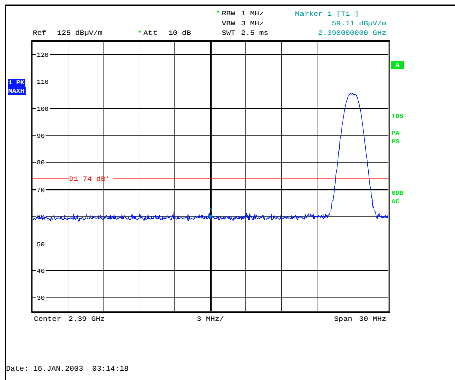
Figure 35 - Static – GFSK/DH5 - 2402 MHz - Measured Frequency 2390.0 MHz - Peak
