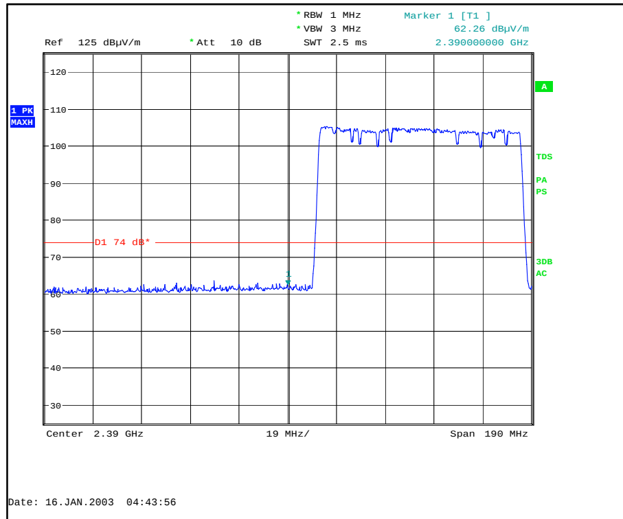
Figure 49 - Hopping - \pi/4 DQPSK/2DH5 - Measured Frequency 2390.0 MHz - Peak
