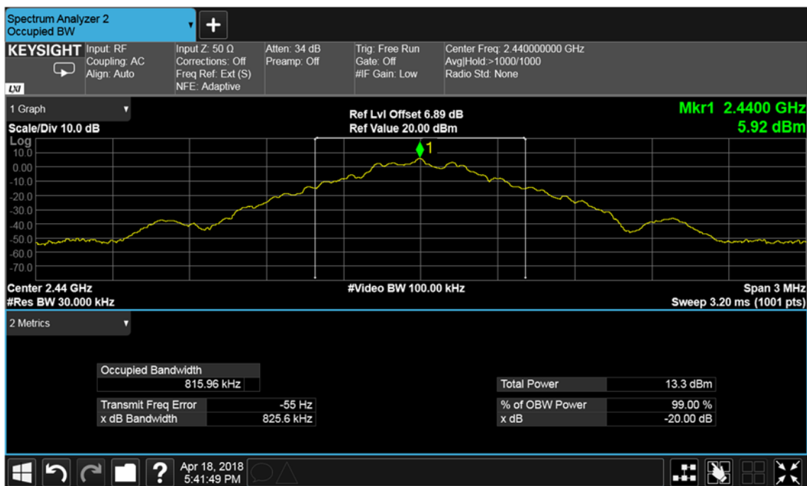
Figure 17 – 2440 MHz - GFSK
