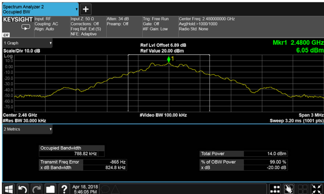
Figure 20 – 2480 MHz - GFSK
