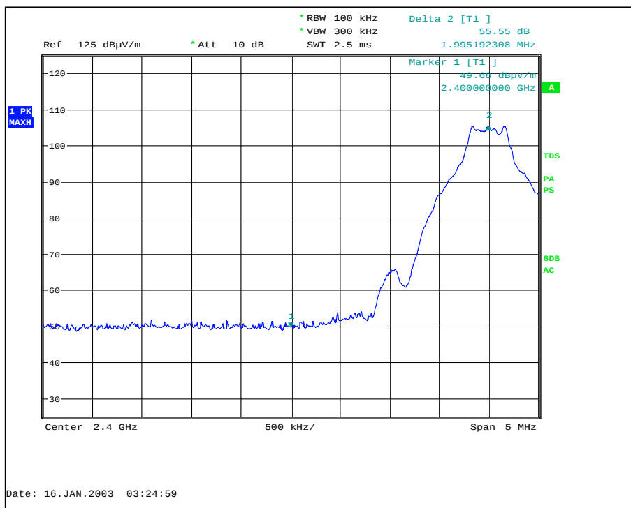
Figure 23 - Static – GFSK/DH5 - 2402 MHz - Measured Frequency 2400.0 MHz
