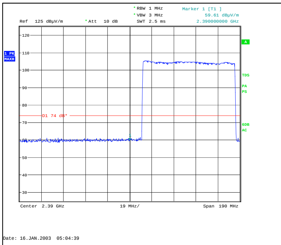
Figure 47 - Hopping - GFSK/DH5 - Measured Frequency 2390.0 MHz - Peak
