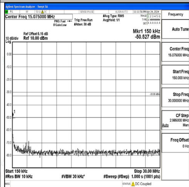
Band4_1.4MHz_QPSK_20175_1RB#0_0.15~30_0.15~30
