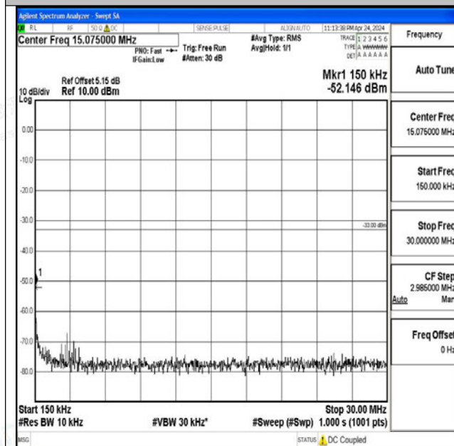
Band4_1.4MHz_16QAM_20393_1RB#0_0.15~30_0.15~ 30
