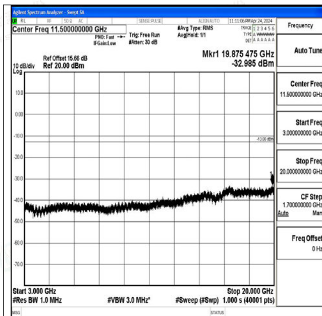
Band4_1.4MHz_QPSK_19957_1RB#0_3000~20000_300 0~20000
