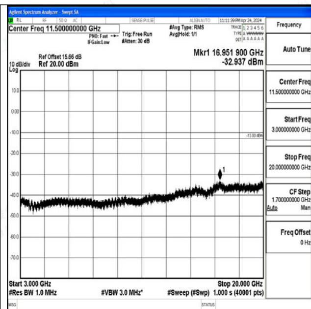
Band4_1.4MHz_16QAM_19957_1RB#0_3000~20000_3 000~20000
