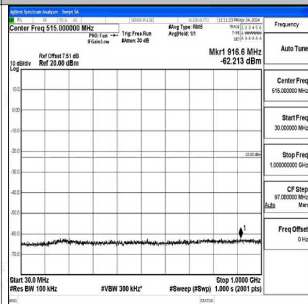
Band4_1.4MHz_16QAM_19957_1RB#0_30~1000_30~1000 000
