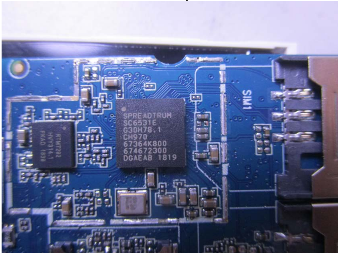
Main Chip
