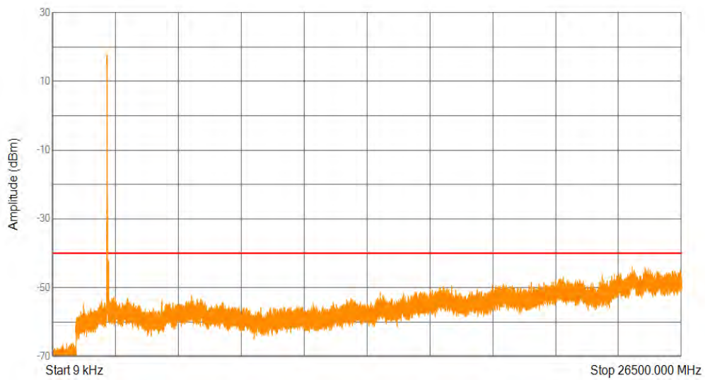
Band40(2305-2315) QAM16 BW=10MHz Channel=38750 RB Size=50 Position=#0
