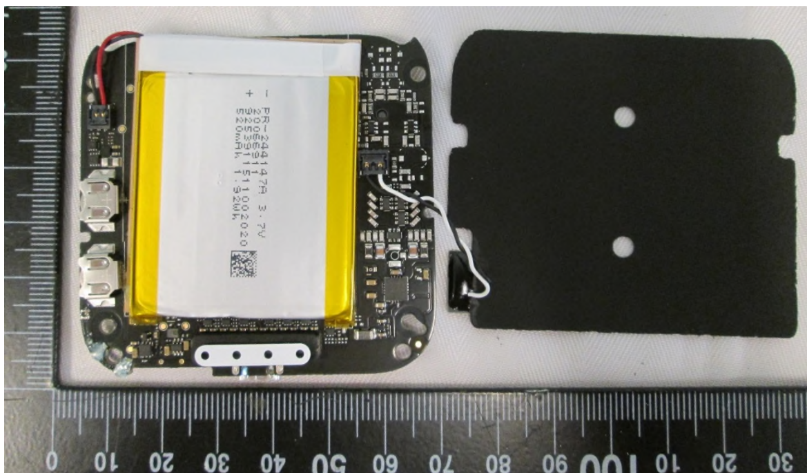
EUT – Internal view 7 Close-up of PCB side 2.
