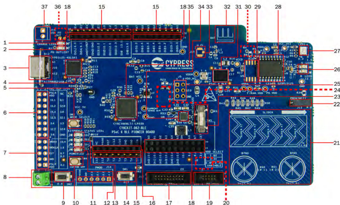
Figure 3-4. PSoC 6 BLE Pioneer board - Top View
