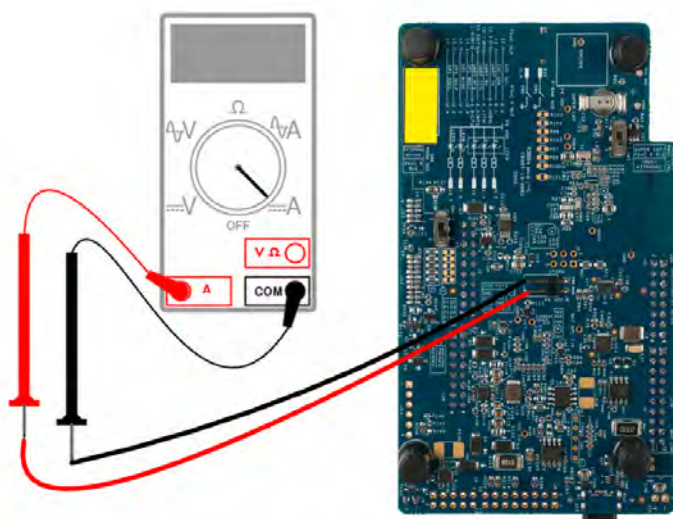
Figure A-15. Jumper J8 on board
