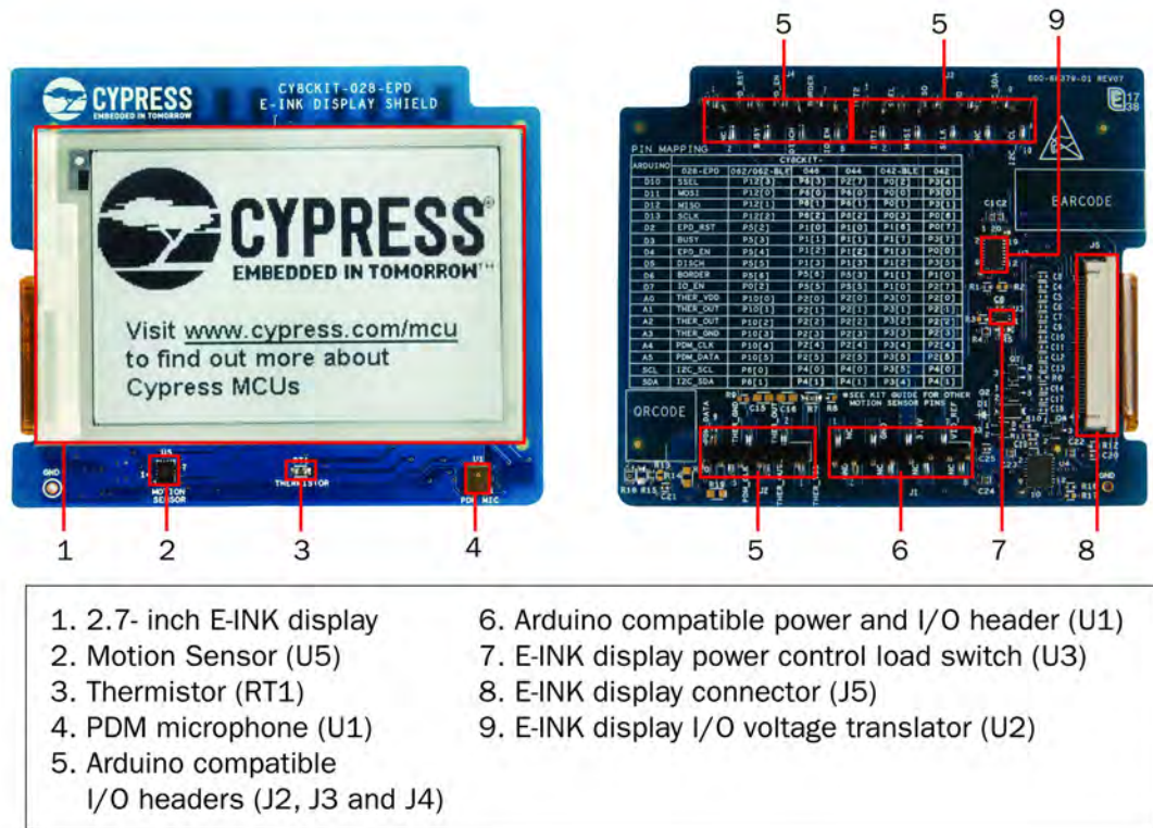
Figure 1-4. E-INK Display Shield
