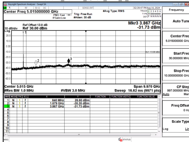
Band26_10MHz_QPSK_RB1_0_CH26990
