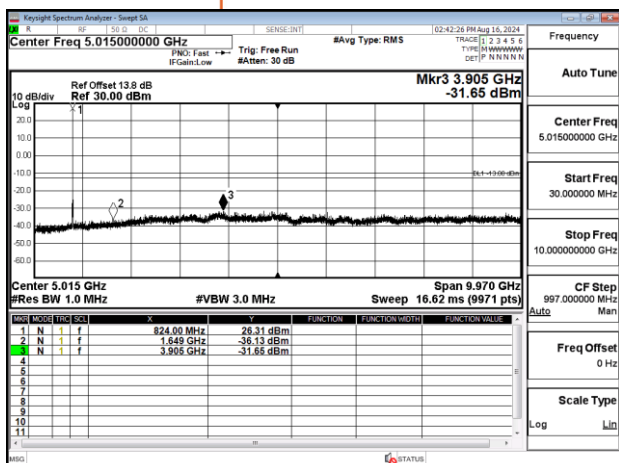
Band26_5MHz_QPSK_RB1_0_CH26915
