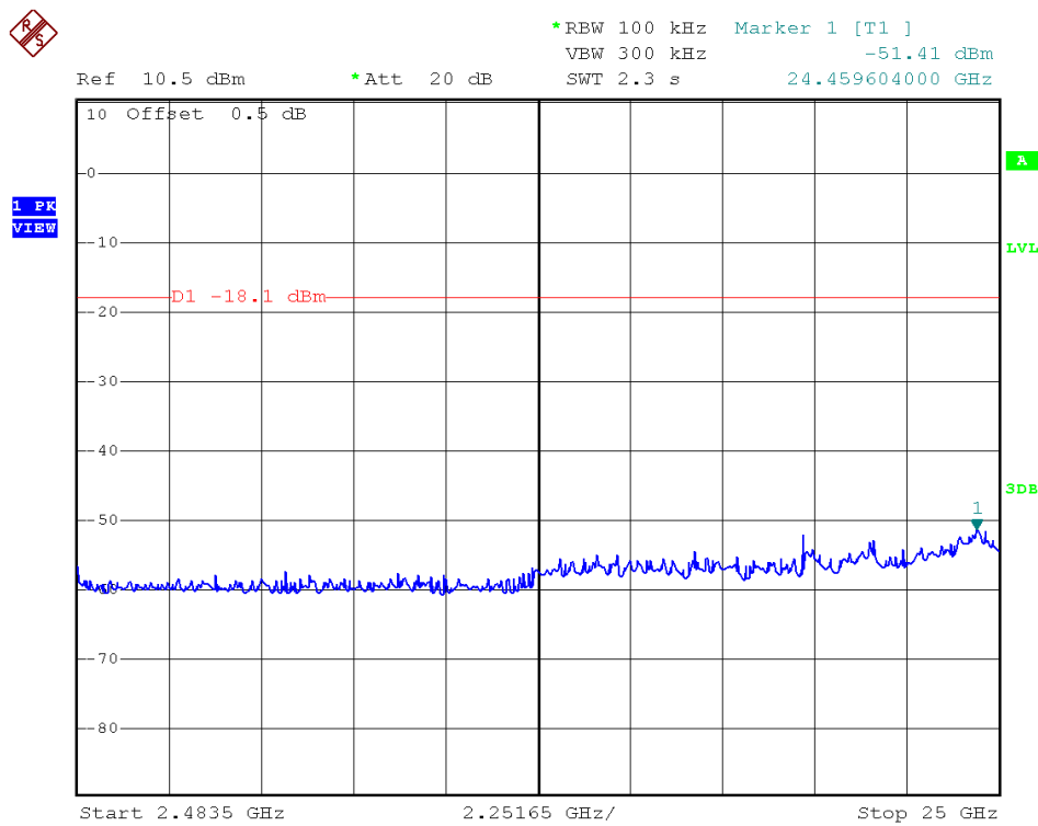
802.11b, Highest Channel, Plot B
