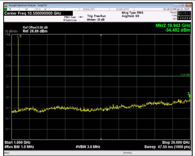
Band66-1.4MHz-QPSK-132665-1RB#0-Range2:1000 ~20000MHz
