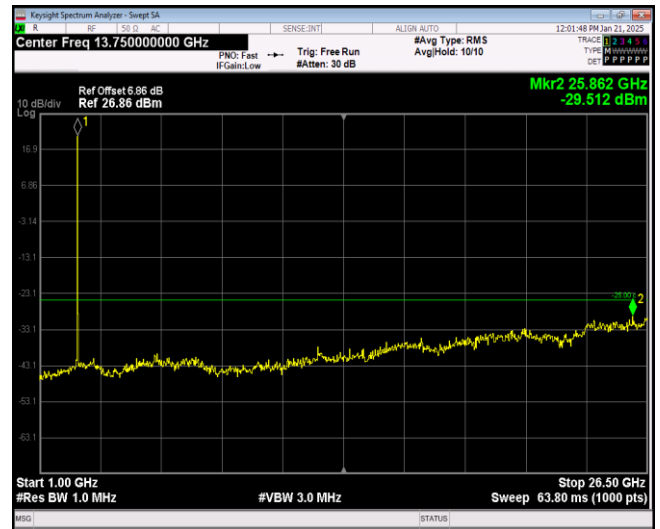
Band38-5MHz-64QAM-38225-1RB#0-Range2:1000~26500MHz
