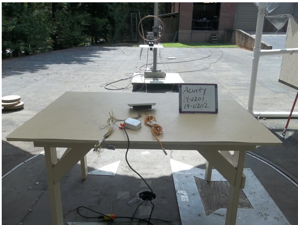
Photo 5- Radiated Emissions Test Setup, below 30 MHz, Back
