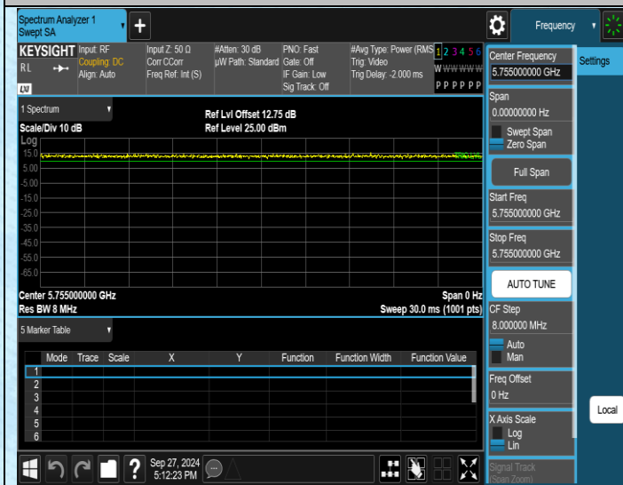
NTNV-11N40SISO-Ant1-5755
