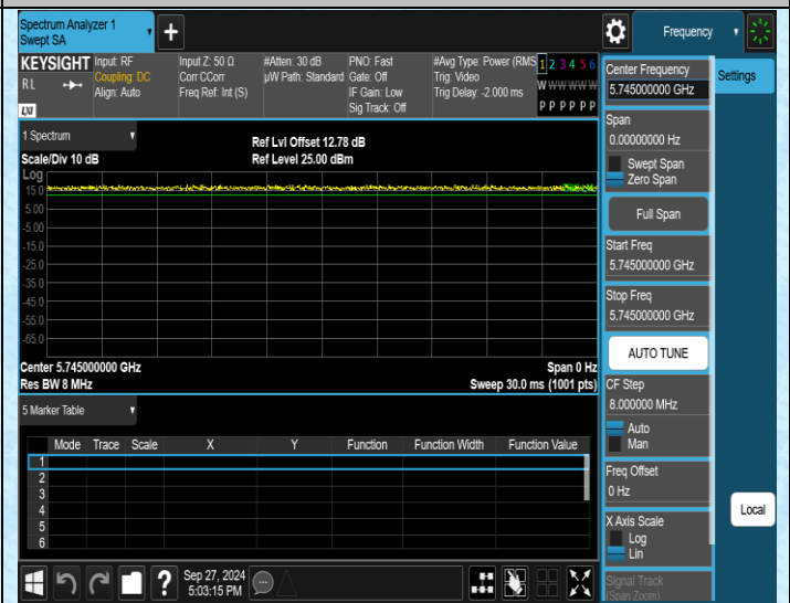
NTVN-11N20SISO-Ant1-5745
