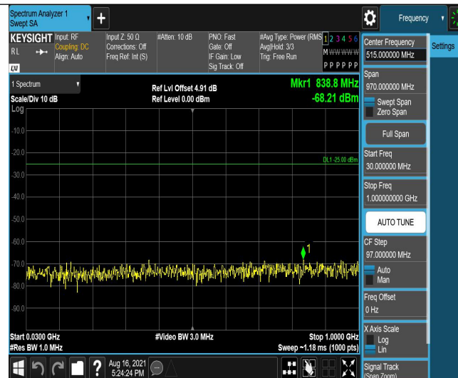
Band7-5MHz-16QAM-20775-25RB#0-Range1:30~1000MHz
