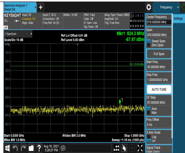
Band7-5MHz-16QAM-21425-25RB#0-Range1:30~1000MHz
