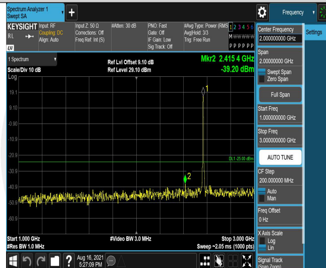
Band7-5MHz-16QAM-21425-25RB#0-Range2:1000~3000MHz
