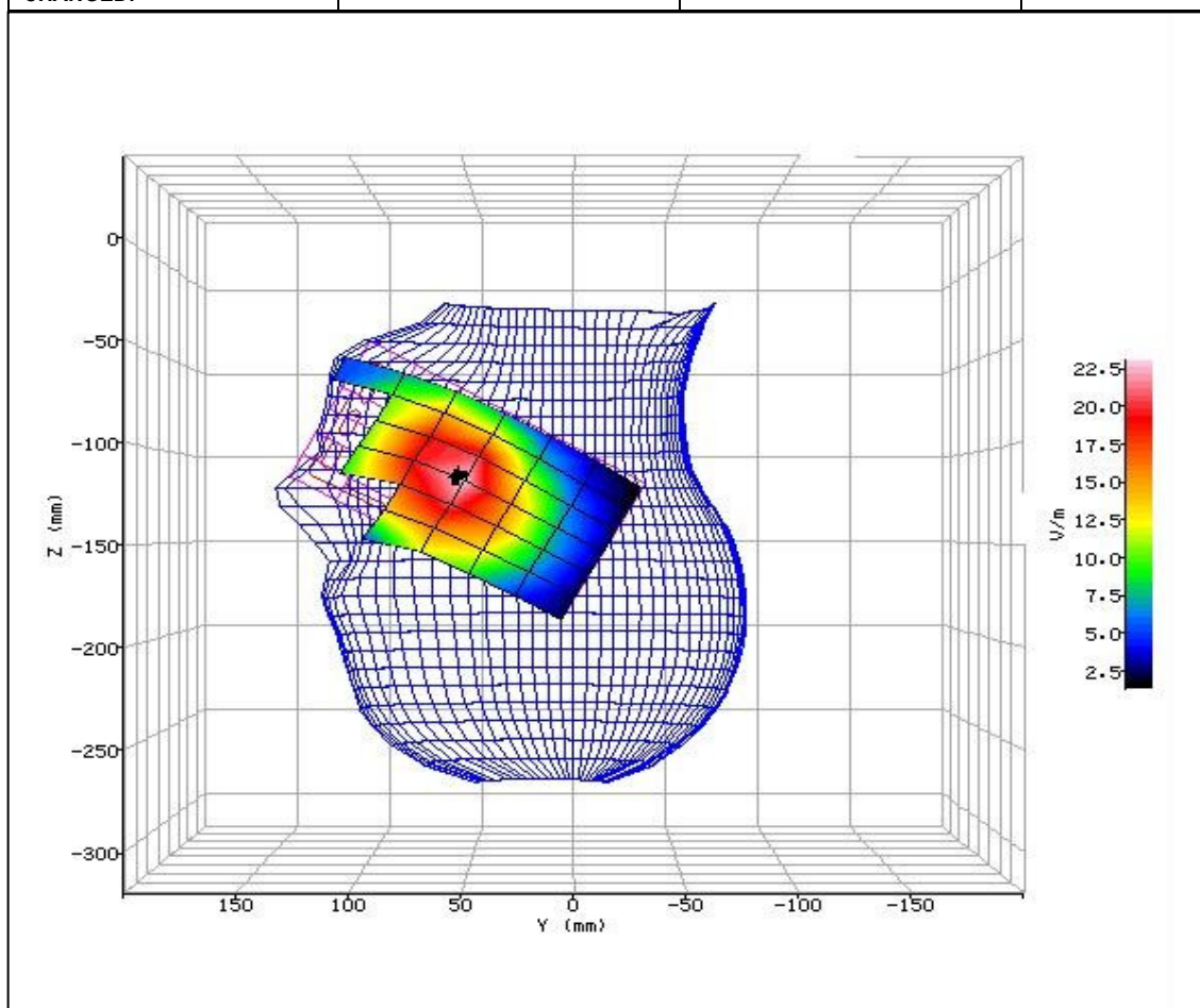
Figure 10: SAR Head Testing Results for the Mobile Handset at 836.4MHz.
