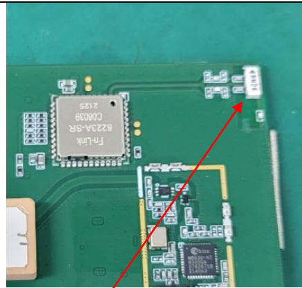
Chip Antenna
