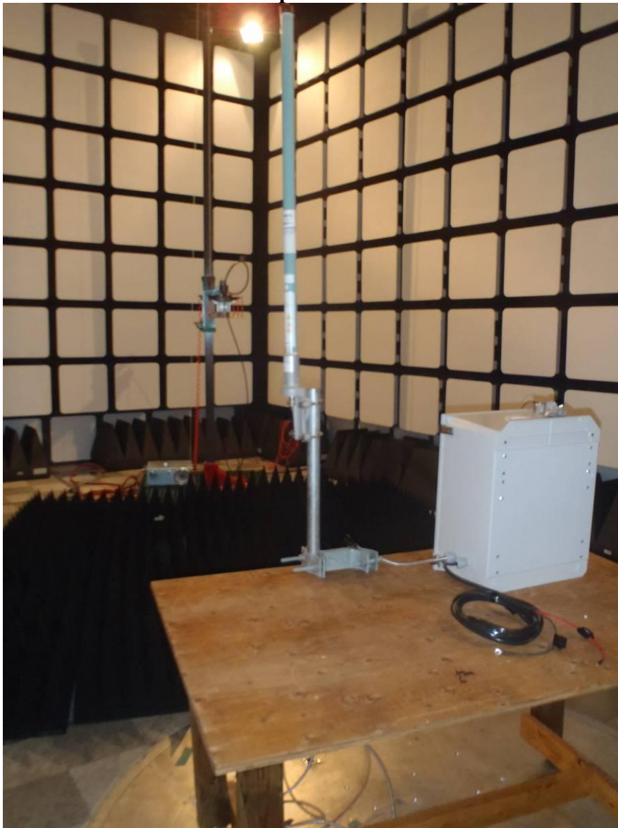
Radiated Emission Test Setup Photo#1:
