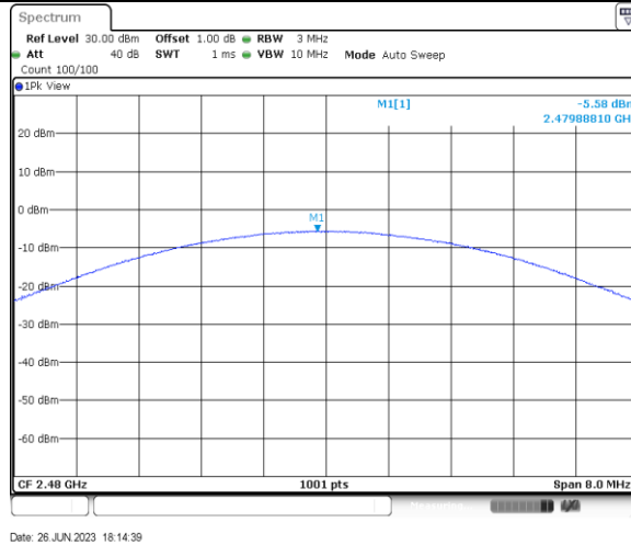
3DH5_Ant1_2480
