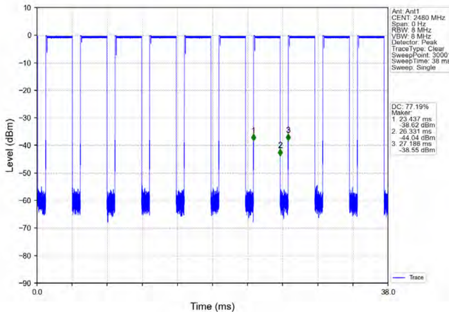
Pi/4DQPSK_2DH5_HCH_2480MHz_Ant1_NTNV
